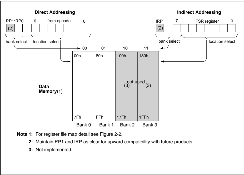
FIGURE 2-11: DIRECT/INDIRECT ADDRESSING
