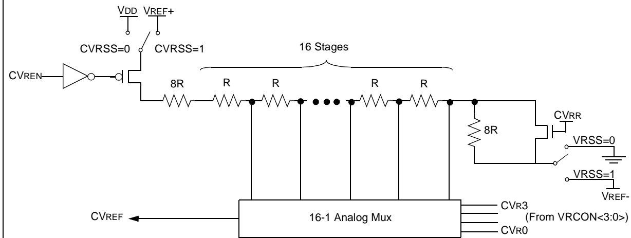
FIGURE 20-1: VOLTAGE REFERENCE BLOCK DIAGRAM
