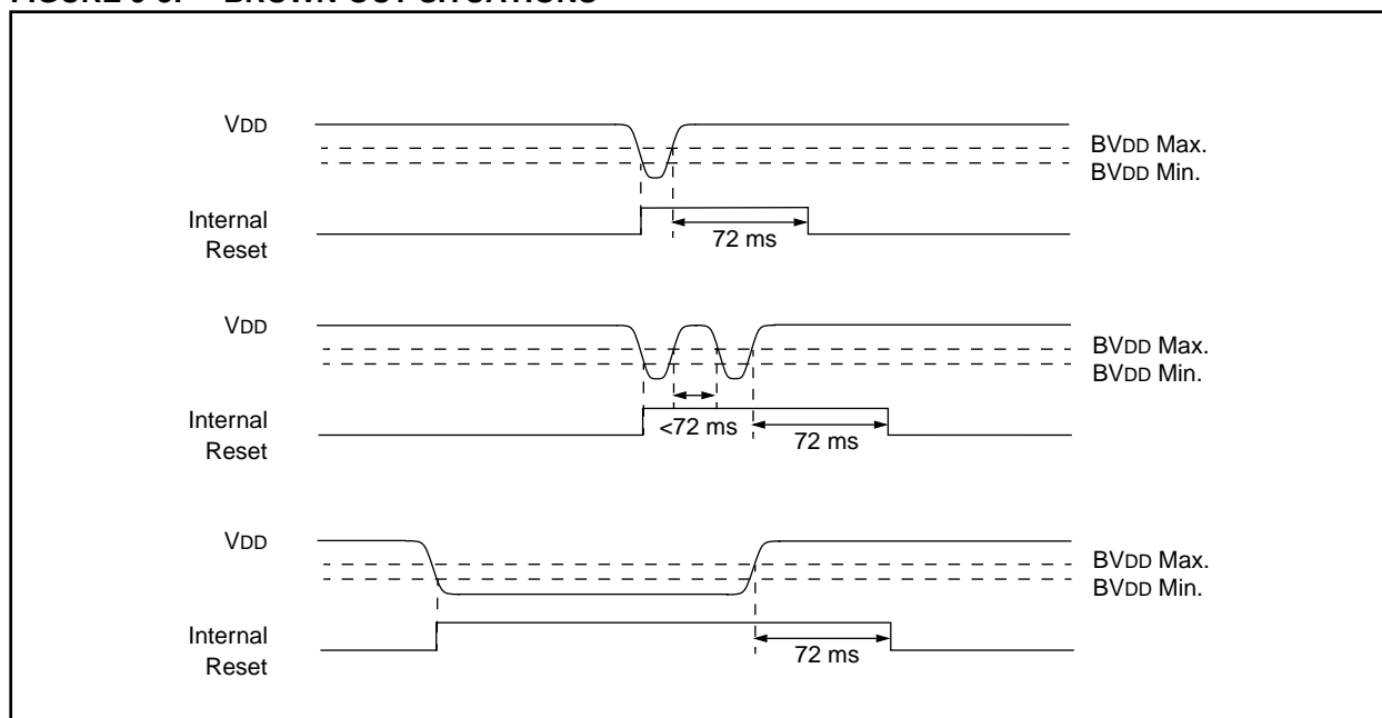
FIGURE 9-8: BROWN-OUT SITUATIONS
