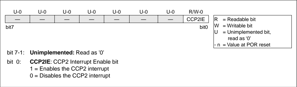
FIGURE 2-8: PIE2 REGISTER (ADDRESS 8Dh)
