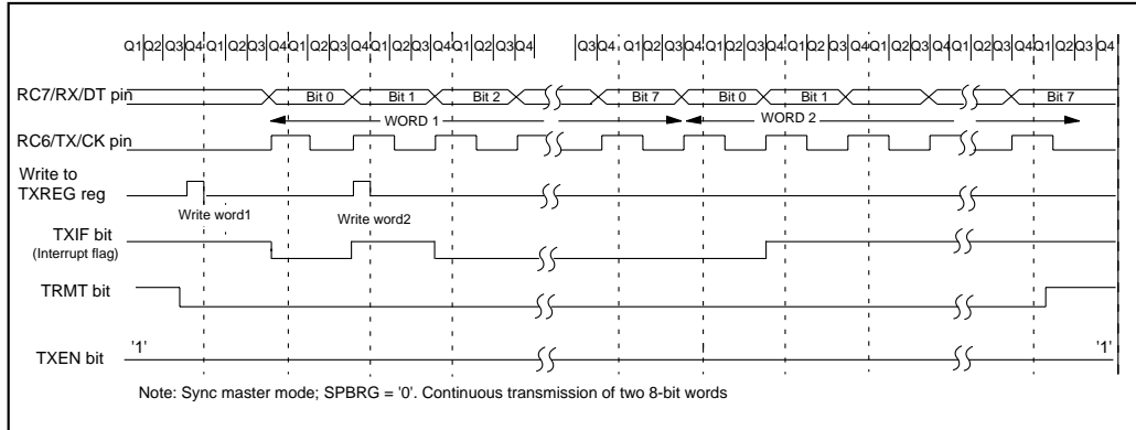
FIGURE 9-8: SYNCHRONOUS TRANSMISSION
