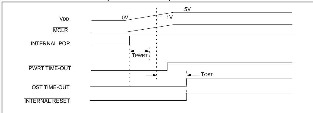
FIGURE 11-10: SLOW RISE TIME ( \overline{\text{MCLR}} TIED TO V_{DD} )
