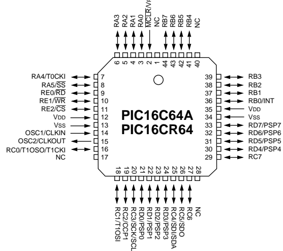
PLCC
