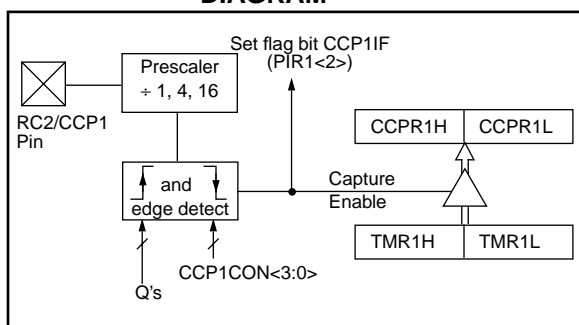
FIGURE 7-2: CAPTURE MODE OPERATION BLOCK DIAGRAM
