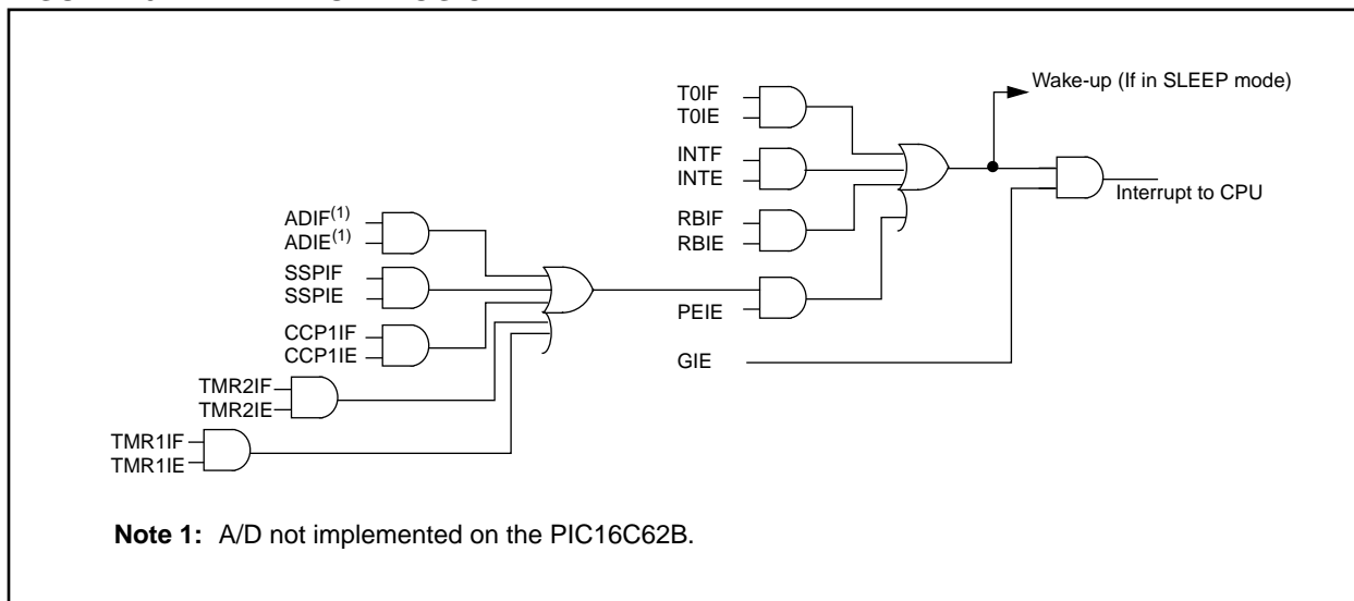
FIGURE 10-11: INTERRUPT LOGIC
