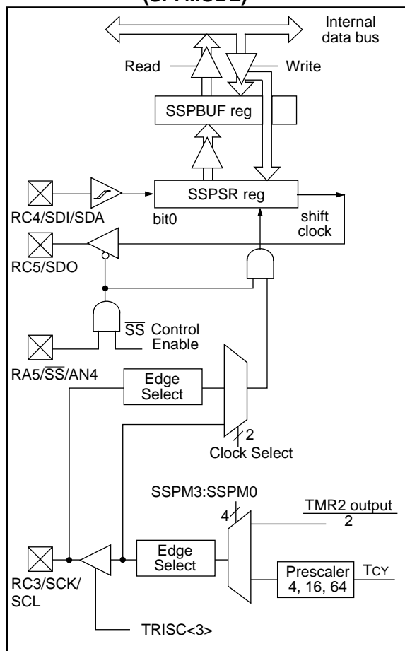
FIGURE 8-3: SSP BLOCK DIAGRAM (SPI MODE)
