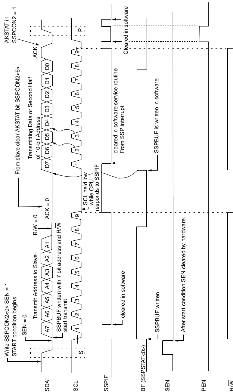
FIGURE 8-26: I 2 C MASTER MODE TIMING (TRANSMISSION, 7 OR 10-BIT ADDRESS)
