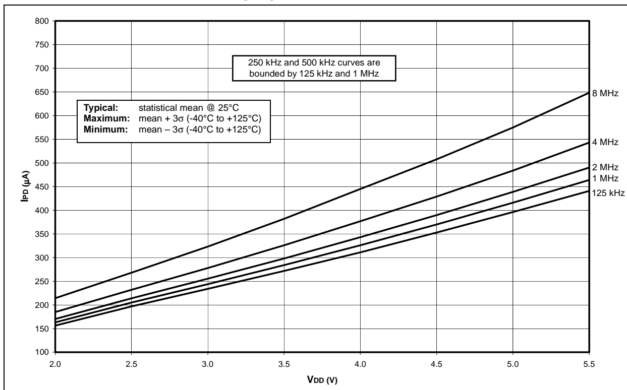
FIGURE 27-18: TYPICAL I_{PD} vs. V_{DD} (+25°C), 125 kHz TO 8 MHz RC_IDLE MODE, ALL PERIPHERALS DISABLED
