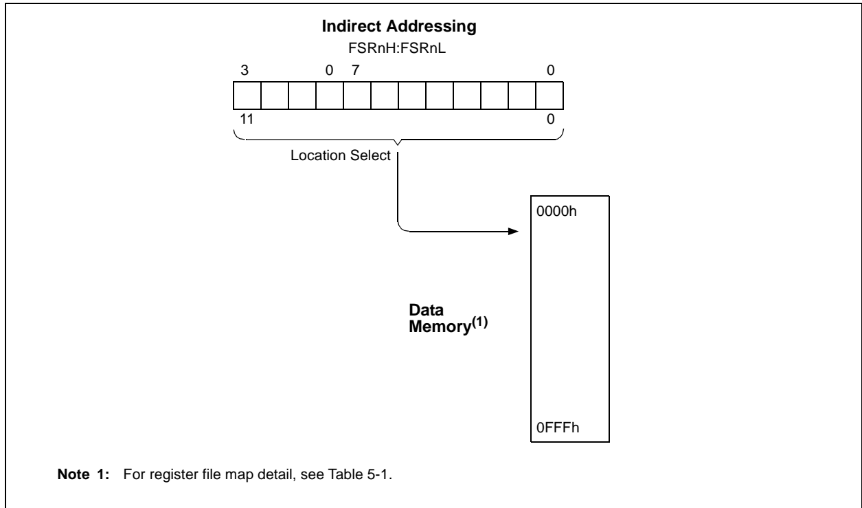
FIGURE 5-9: INDIRECT ADDRESSING
