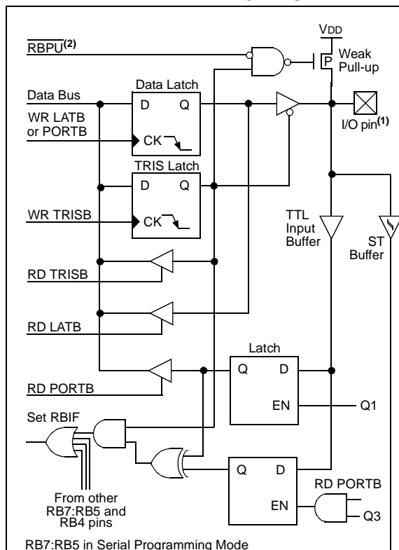
FIGURE 10-6: BLOCK DIAGRAM OF RB7:RB5 PINS
