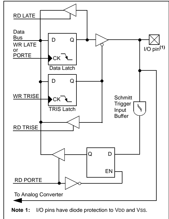
FIGURE 10-13: BLOCK DIAGRAM OF RE2:RE0 PINS
