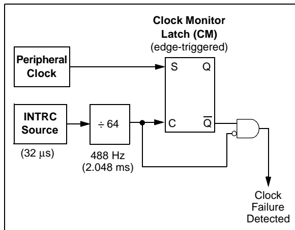
FIGURE 23-3: FSCM BLOCK DIAGRAM
