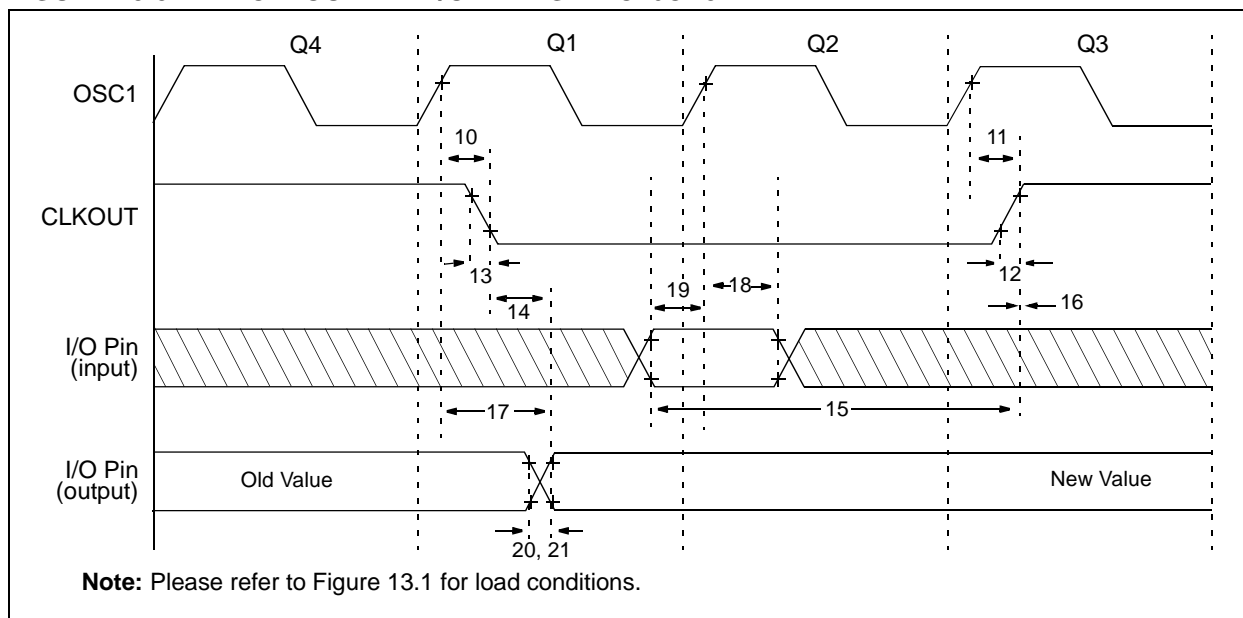
FIGURE 13-3: CLKOUT AND I/O TIMING - PIC16CR54A
