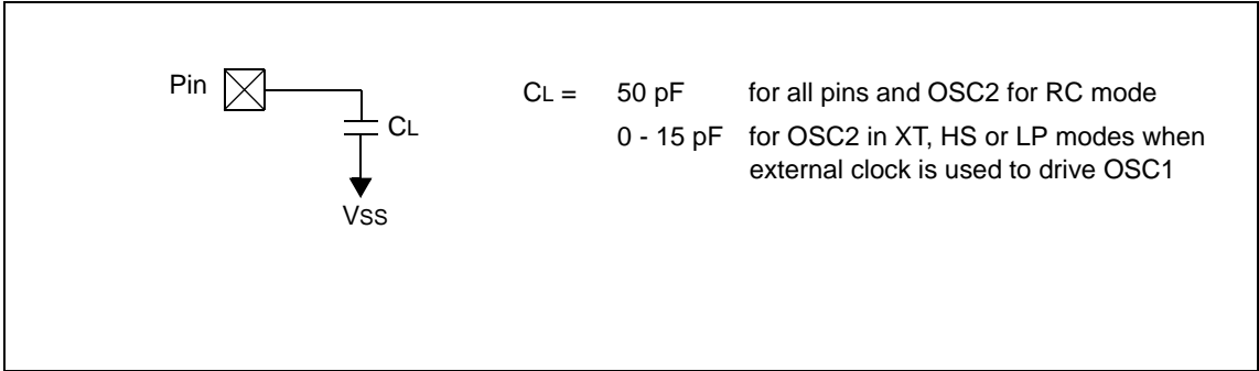
FIGURE 12-1: LOAD CONDITIONS FOR DEVICE TIMING SPECIFICATIONS - PIC16C54/55/56/57
