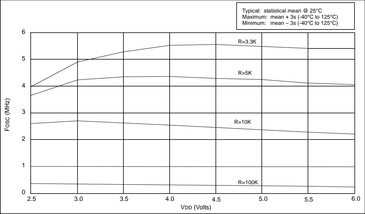
FIGURE 16-3: TYPICAL RC OSCILLATOR FREQUENCY vs. VDD, CEXT = 100 pF, 25°C
