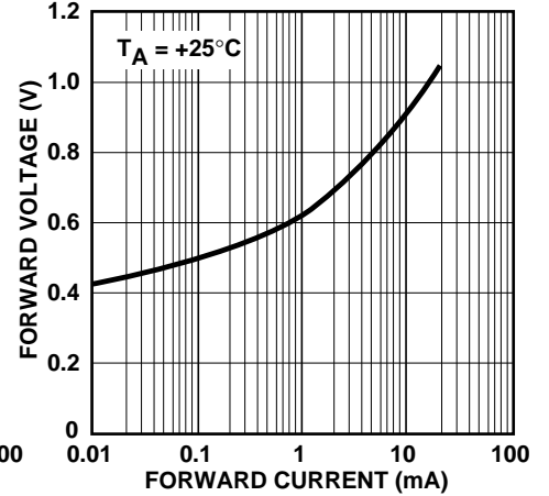
TC04: Forward Voltage vs Forward Current
