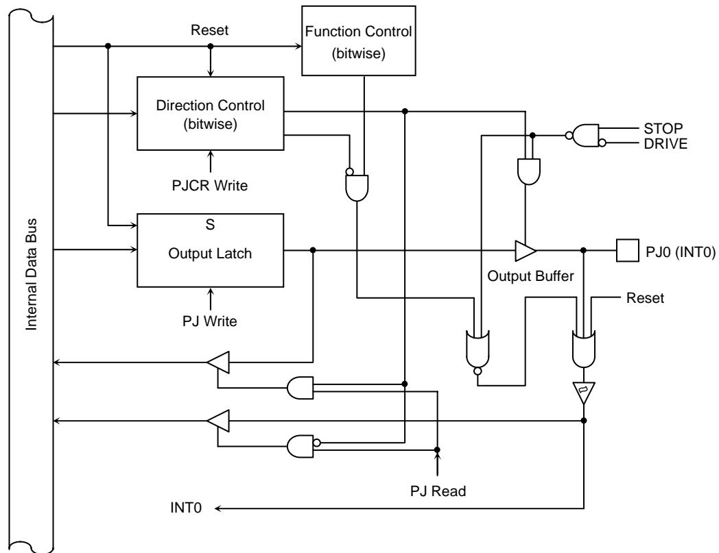
Figure 7.56 Port J (PJ0)
