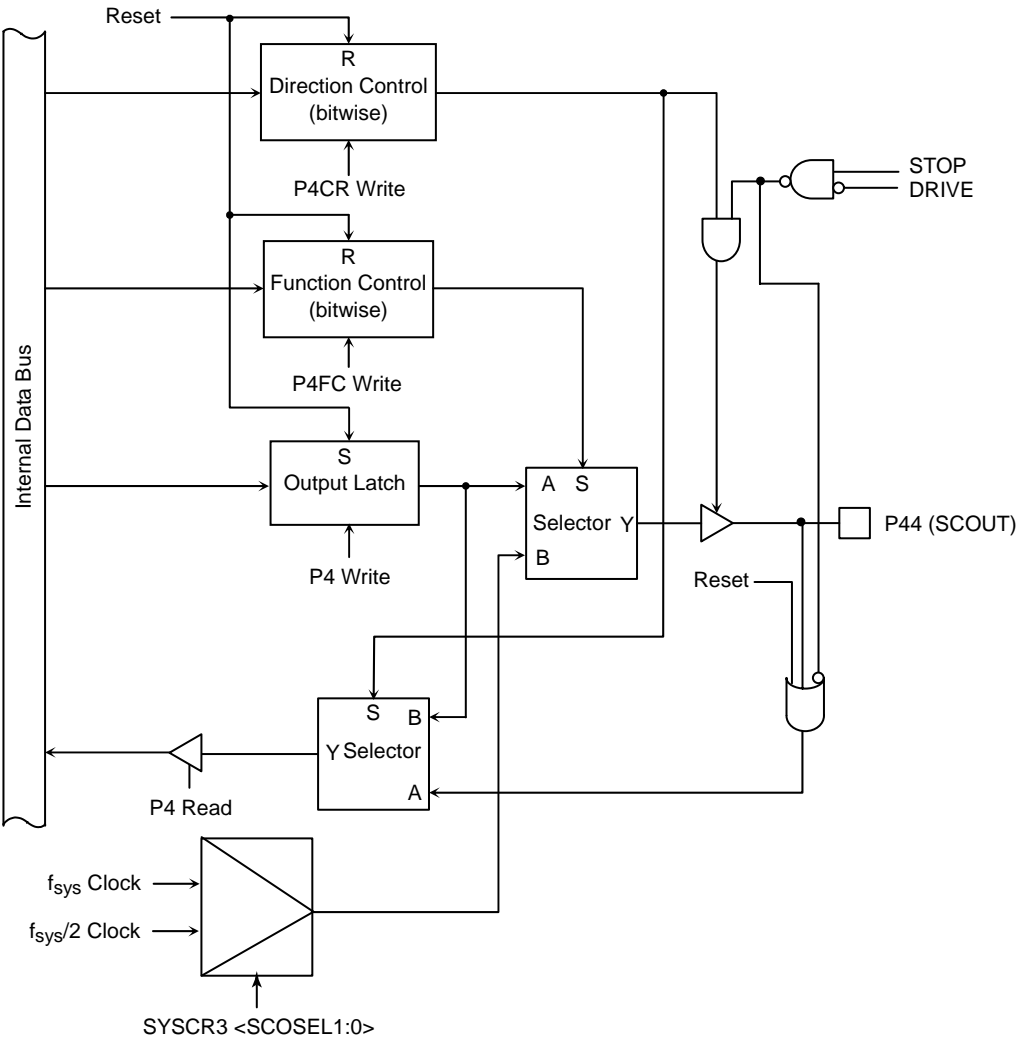
Figure 7.13 Port 4 (P44)
