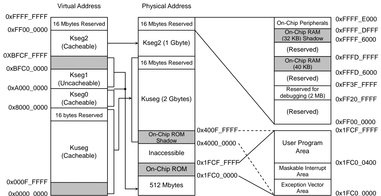
Figure 0.1 Memory Map
