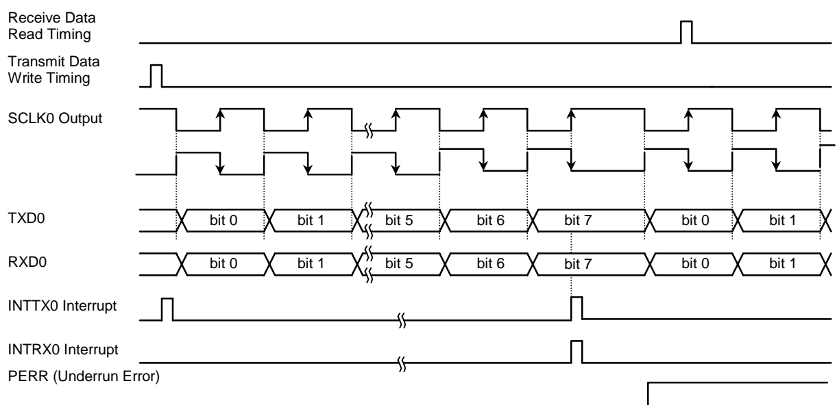
Figure 14.17 Full-Duplex Transmit/Receive Operation in I/O Interface Mode (SCLK0 Input Mode)
