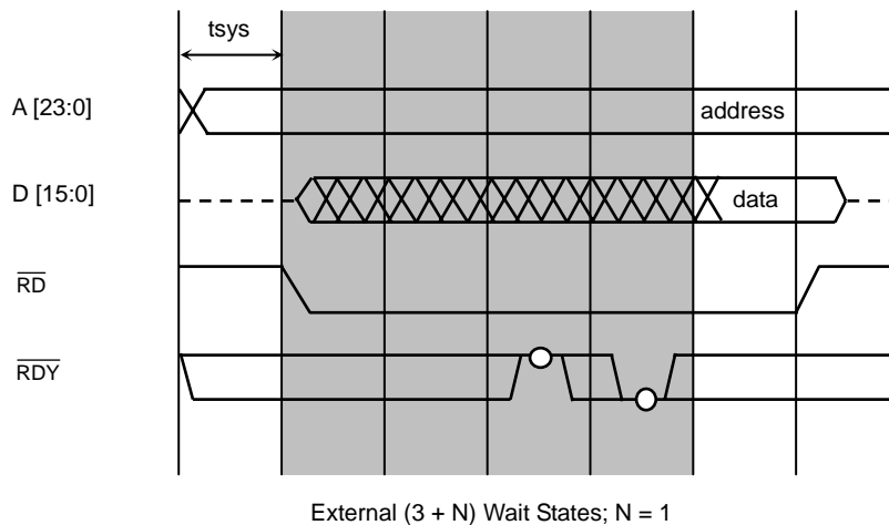
Figure 8.14 \overline{\text{RDY}} Input Timing (with Externally Inserted (3 + N) Wait States; N = 1)
