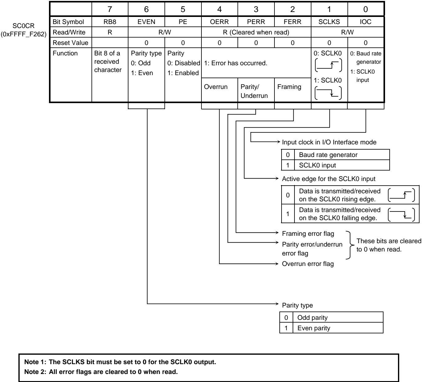
Figure 14.9 Serial Control Register (SC0CR, for SIO0)
