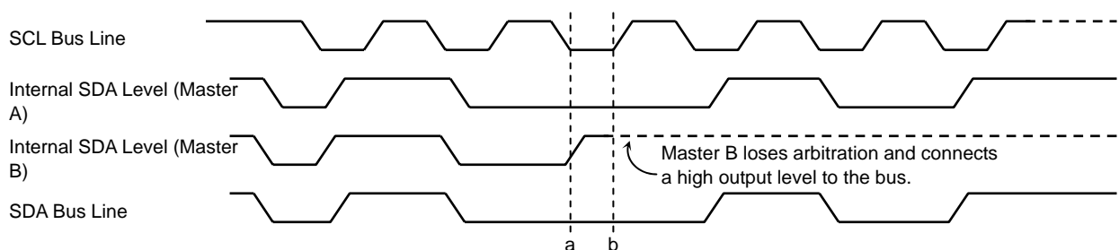
Figure 15.12 Arbitration Procedure of Two Masters
