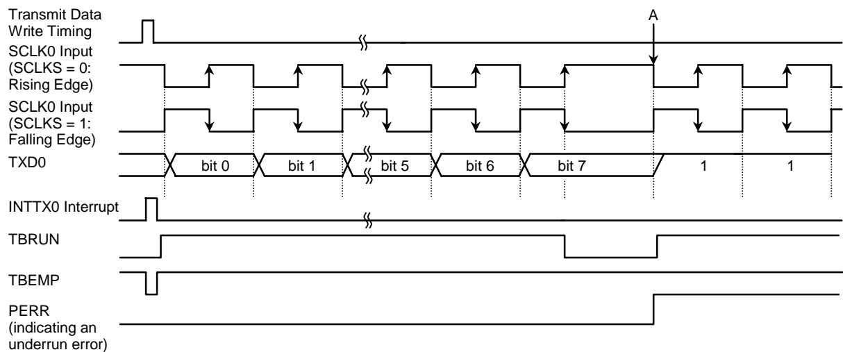
Figure 14.13 Transmit Operation in I/O Interface Mode (SCLK0 Input Mode)
