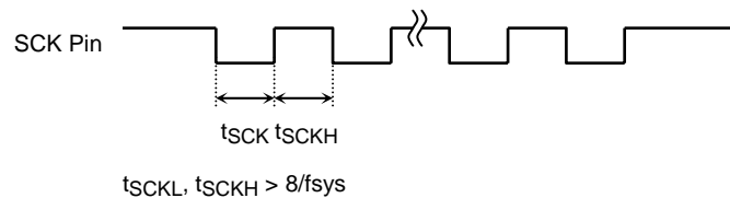
Figure 15.23 Maximum External Clock Frequency
