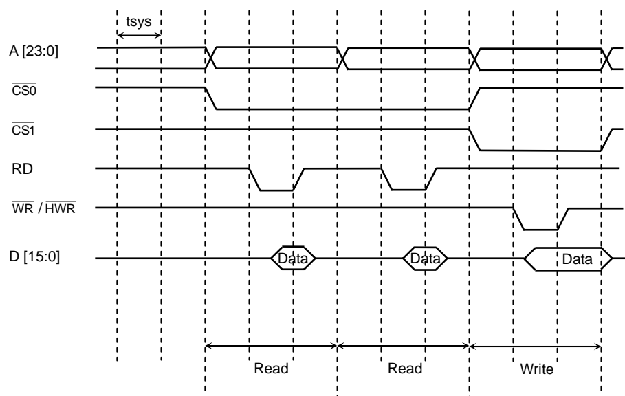
Figure 10.18 I/O-to-Memory Transfer (Dual-Address Mode)
