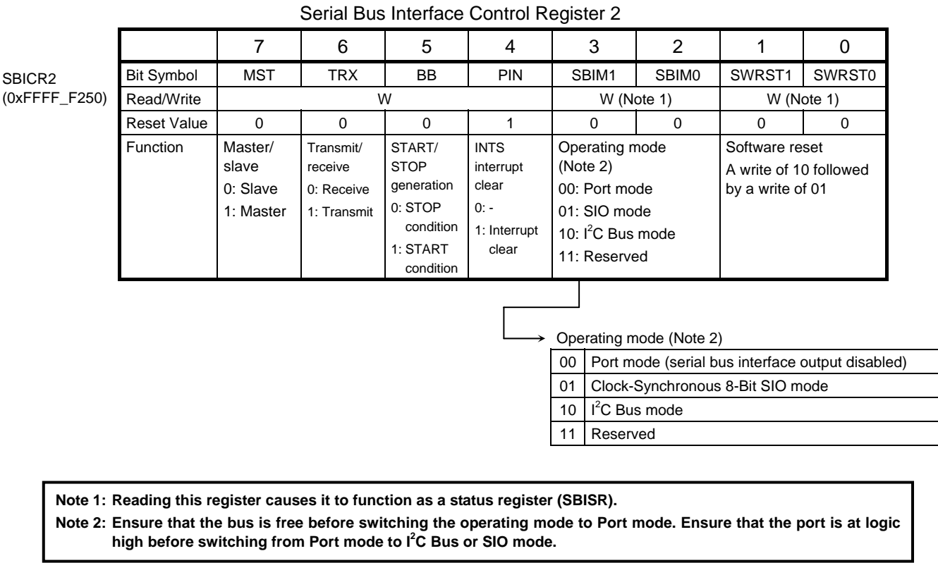
Figure 15.5 I 2 C Bus Mode Registers
