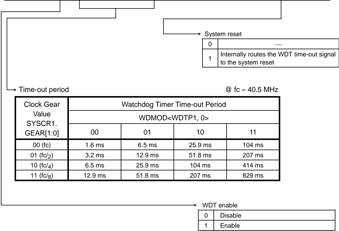
Figure 17.4 Watchdog Timer Mode Register
