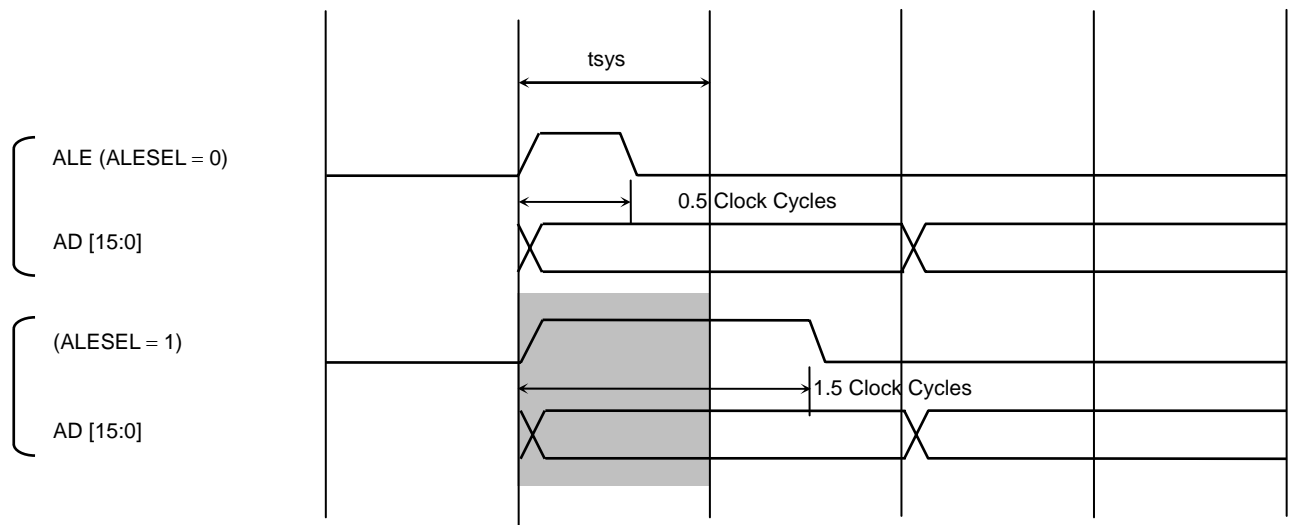
Figure 8.30 ALE Pulse Width
