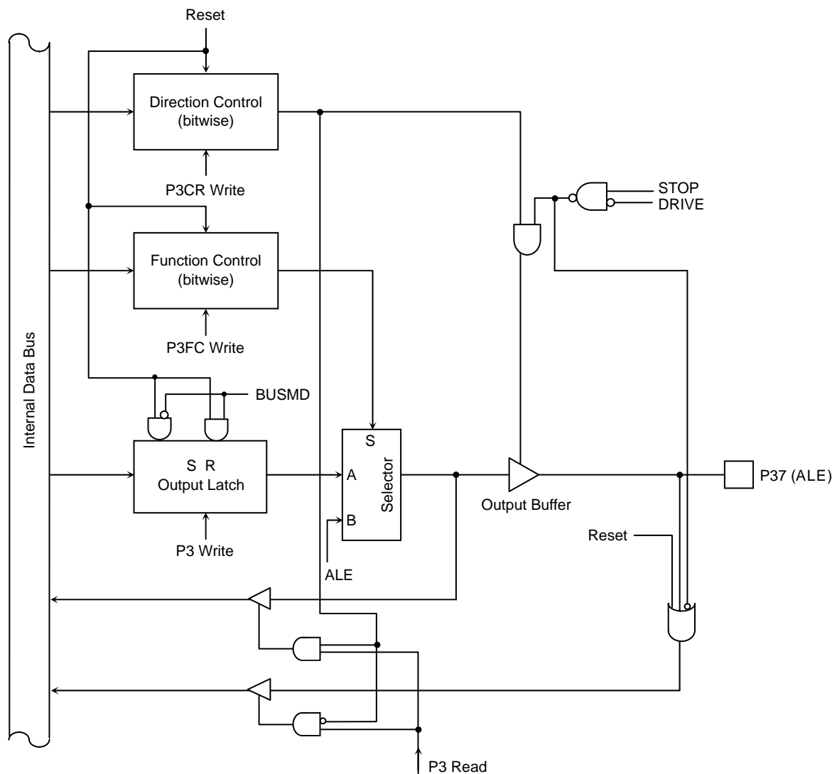
Figure 7.10 Port 3 (P37)
