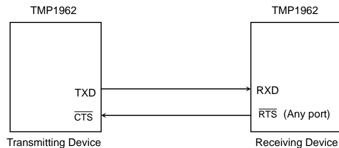
Figure 14.4 Handshaking Signals
