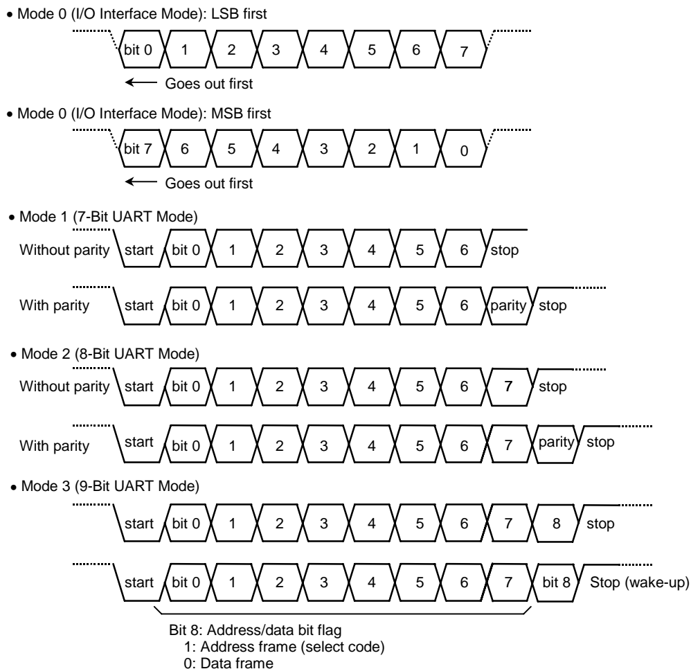
Figure 14.1 Data Formats
