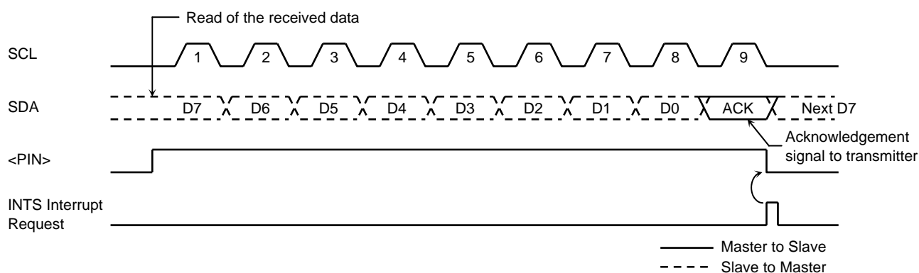
Figure 15.16 SBICR1.BC[2:0] = 000 and SBICR1.ACK = 1 (Master-Receiver Mode)
