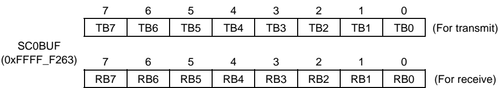
Figure 14.11 Serial Transmit/Receive Buffer Register (SC0BUF, for SIO0)
