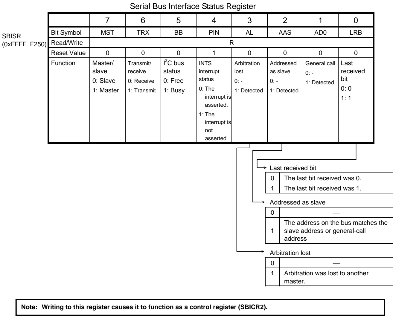
Figure 15.6 I 2 C Bus Mode Registers
