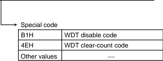
Figure 17.5 Watchdog Timer Control Register
