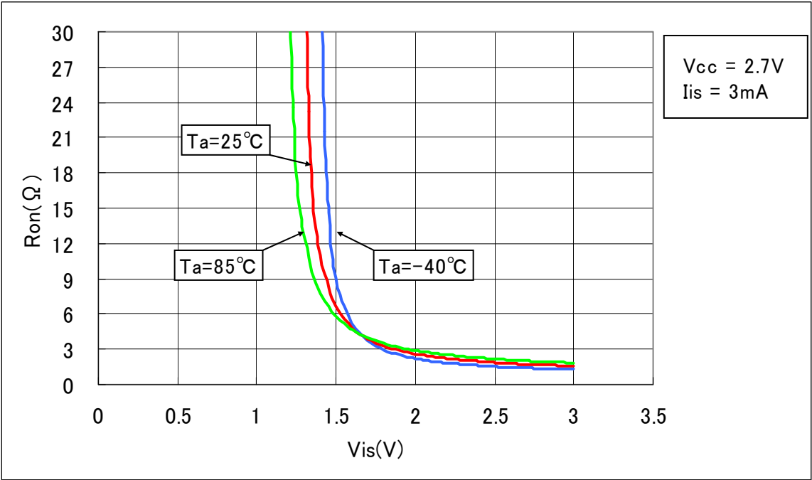
R_{ON} - V_{IN} Characteristic Curves V_{CC} = 2.7 V , I_{is} = 3 mA , T_a = -40/25/85^{\circ}C
