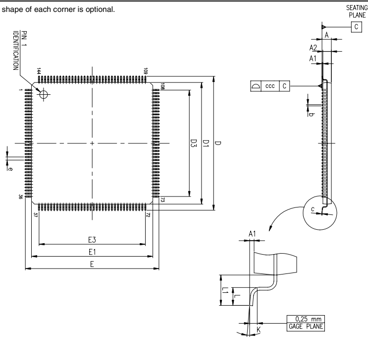
LQFP144 (20x20x1.40mm)
