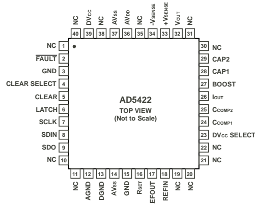
Figure 6. LFCSP Pin Configuration
