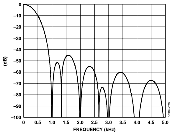
Figure 22. Modified Sinc3 Digital Filter Response at f_{\text{ADC}} = 1.0 \text{ kHz} (ADCFLT = 0x0087)
