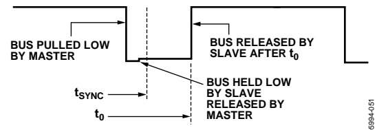
Figure 53. BSD Slave Transmitting Zero
