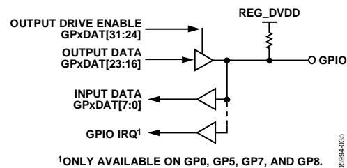
Figure 37. ADuC7034 GPIO
