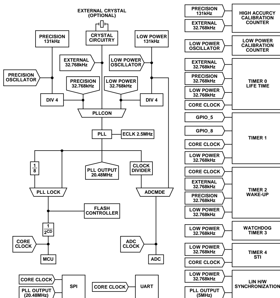
Figure 29. ADuC7034 System Clock Generation
