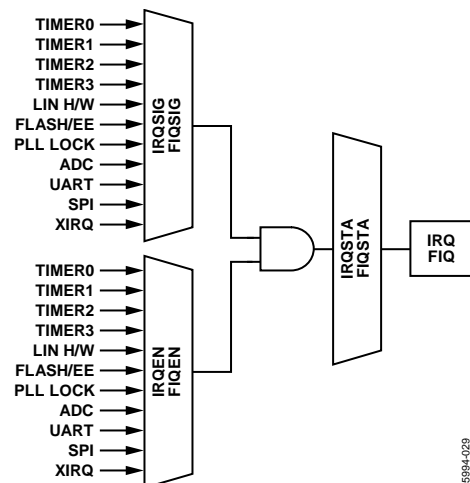
Figure 31. Interrupt Structure
