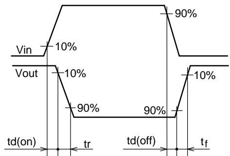
Waveform
