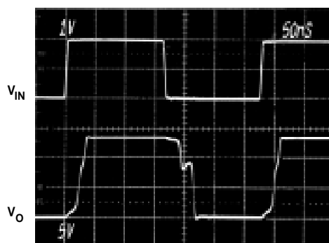
Figure 33. 50% Overload Recovery, Gain = +10, (R_F = 300 \Omega, R_L = 1 kΩ, V_S = \pm 7.5 V)
