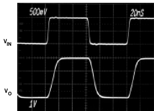
Figure 32. Pulse Response Driving a Large Load Capacitor. C_L = 300 pF, G = +3 , R_F = 750 \Omega , R_S = 16.9 \Omega , R_L = 10 kΩ
