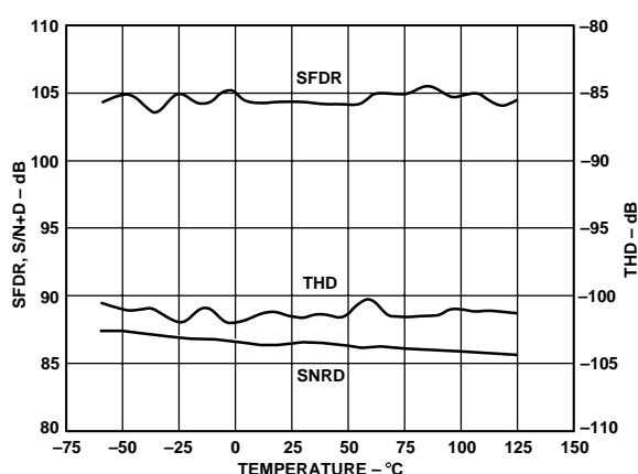
Figure 21. AC Parameters vs. Temperature
