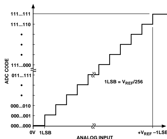
Figure 11. Transfer Characteristic
