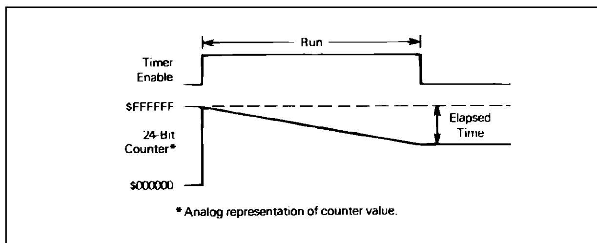
Figure 5.4 : Elapsed Time Measurement Example.
