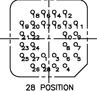
RECOMMENDED CIRCUIT CONFIGURATION VIEWED FROM COMPONENT SIDE OF CIRCUIT
