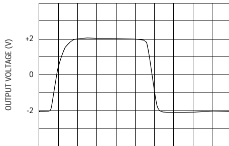
Large Signal Pulse Response (Split Supplies)
