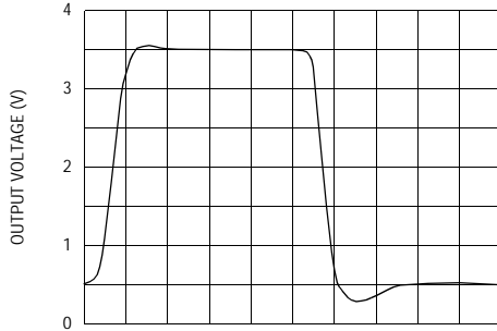
Large Signal Pulse Response (Single Supply)
