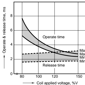
1-(2). Operate & release time (1 Form C type)
