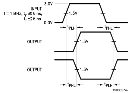
FIGURE 2. Propagation Delays
