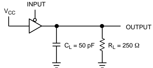
Figure 7. T_{PZH} or T_{PHL}
