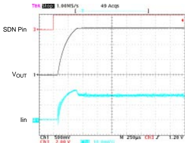
Figure 32. Pulse Startup Inrush Current – 25 \Omega Load, 1.57 V_{out}
