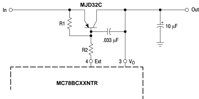
Figure 10. External PNP
