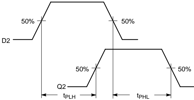
Figure 27. Single-Ended Duty Cycle Skew
