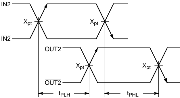
Figure 28. Differential Duty Cycle Skew
