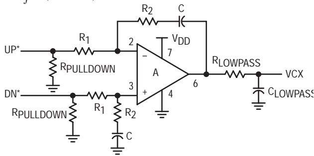
Figure 5-5A. Active Filter Using Op Amp
