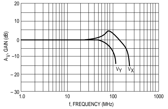
Figure 2. Transconductance Bandwidth
