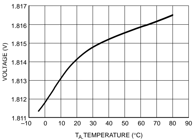
Figure 12. Regulator 1 Line Regulation vs. Temperature 50 mA Load (3.0 V to 3.6 V)
