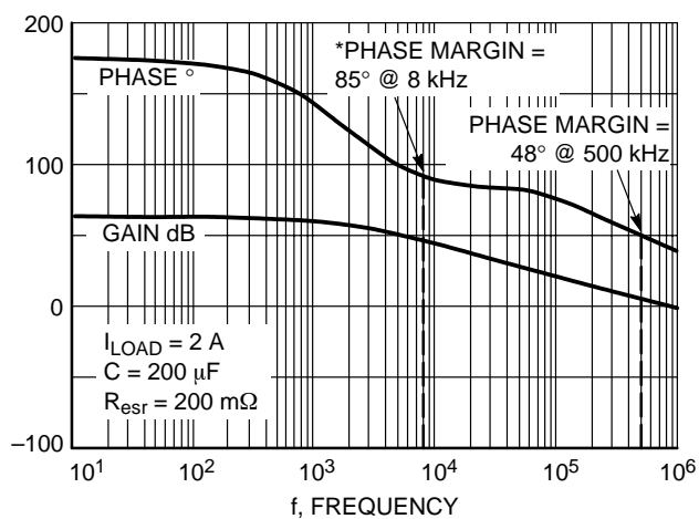
Figure 7. Gain-Phase Plot @ 200 mΩ
