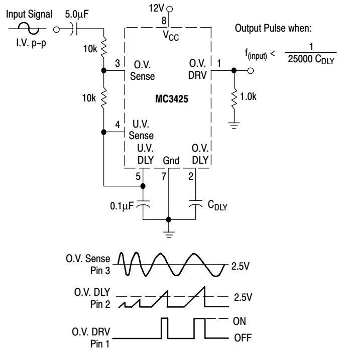
Figure 14. Programmable Frequency Switch
