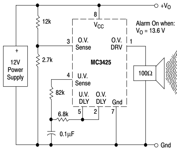
Figure 13. Overvoltage Audio Alarm Circuit
