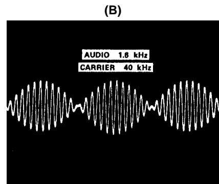
Figure 29. Balanced Modulator
