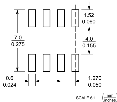
Figure 23. SO-8
