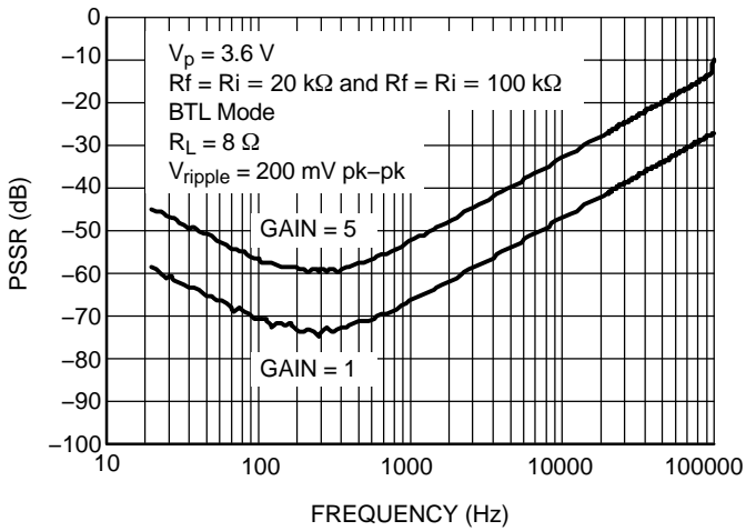
Figure 16. PSSR vs. Gain (BTL Mode) @ V_p = 3.6\text{ V}
