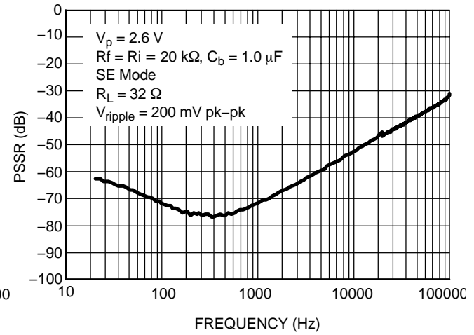
Figure 17. PSSR (SE Mode) @ V_p = 2.6\text{ V}
