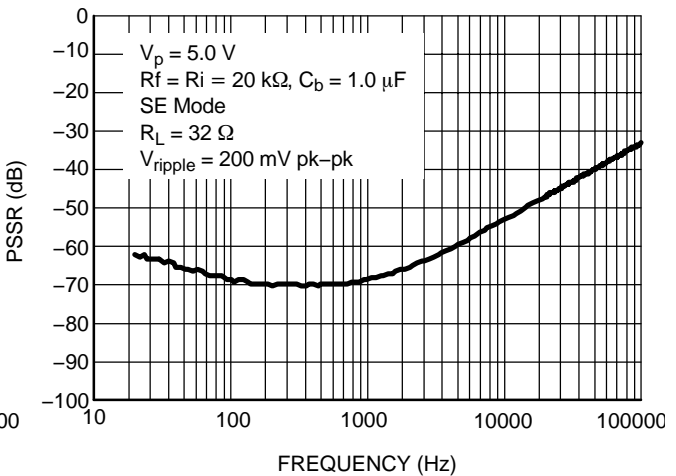
Figure 19. PSSR (SE Mode) @ V_p = 5.0\text{ V}
