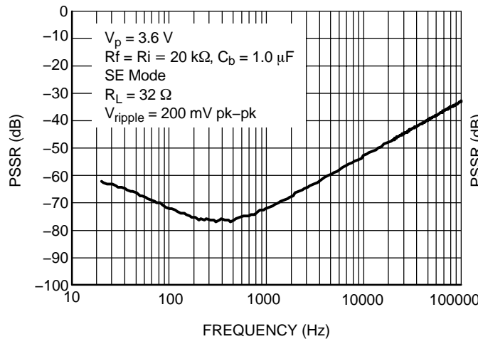
Figure 18. PSSR (SE Mode) @ V_p = 3.6\text{ V}
