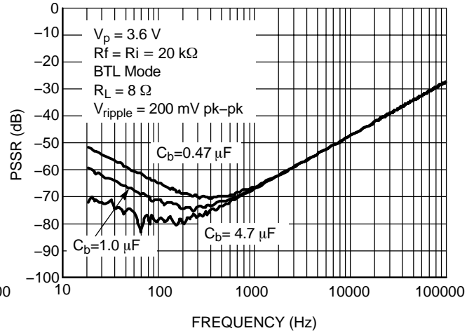
Figure 15. PSSR vs. C_b (BTL Mode) @ V_p = 3.6\text{ V}
