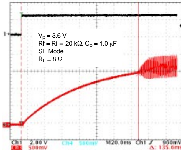
Figure 27. Turn On Sequence (SE Mode) @ V_p = 3.6\text{ V}
