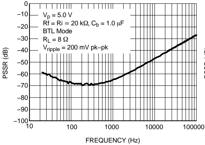
Figure 14. PSSR (BTL Mode) @ V_p = 5.0\text{ V}
