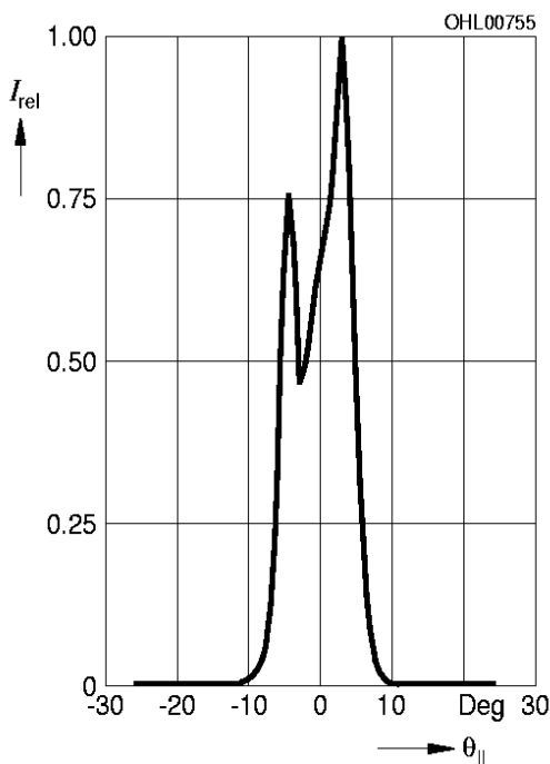
Far-field distribution parallel to junction I_{rel} vs. \theta_{||} ( T_A = 25\text{ }^\circ\text{C} , P_{opt} = 75\text{ W} )
