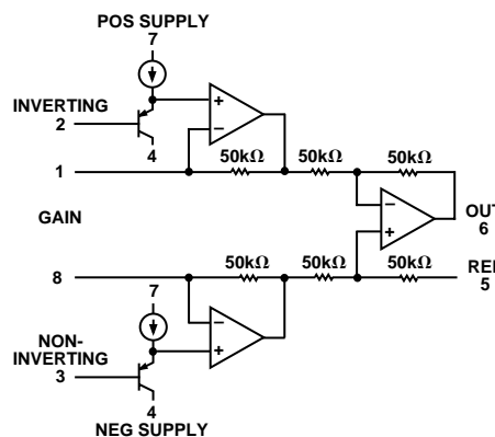
Figure 40. Simplified Schematic
