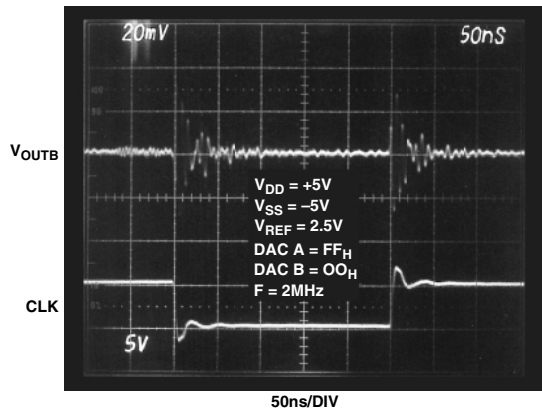
Figure 20. Digital Feedthrough
