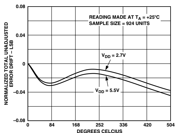
Figure 28. Normalized TUE Drift Accelerated by Burn-In Hours of Operation @ 150^{\circ}C
