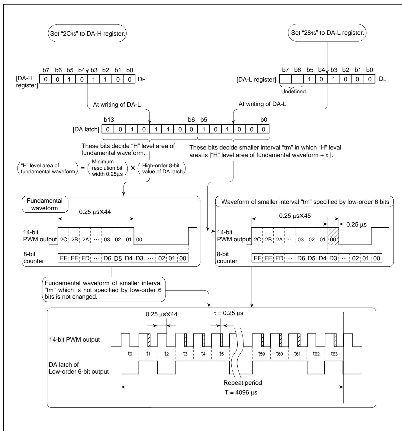
Fig. 15. 14-bit PWM output example ( f(XIN) = 8 \text{ MHz} )
