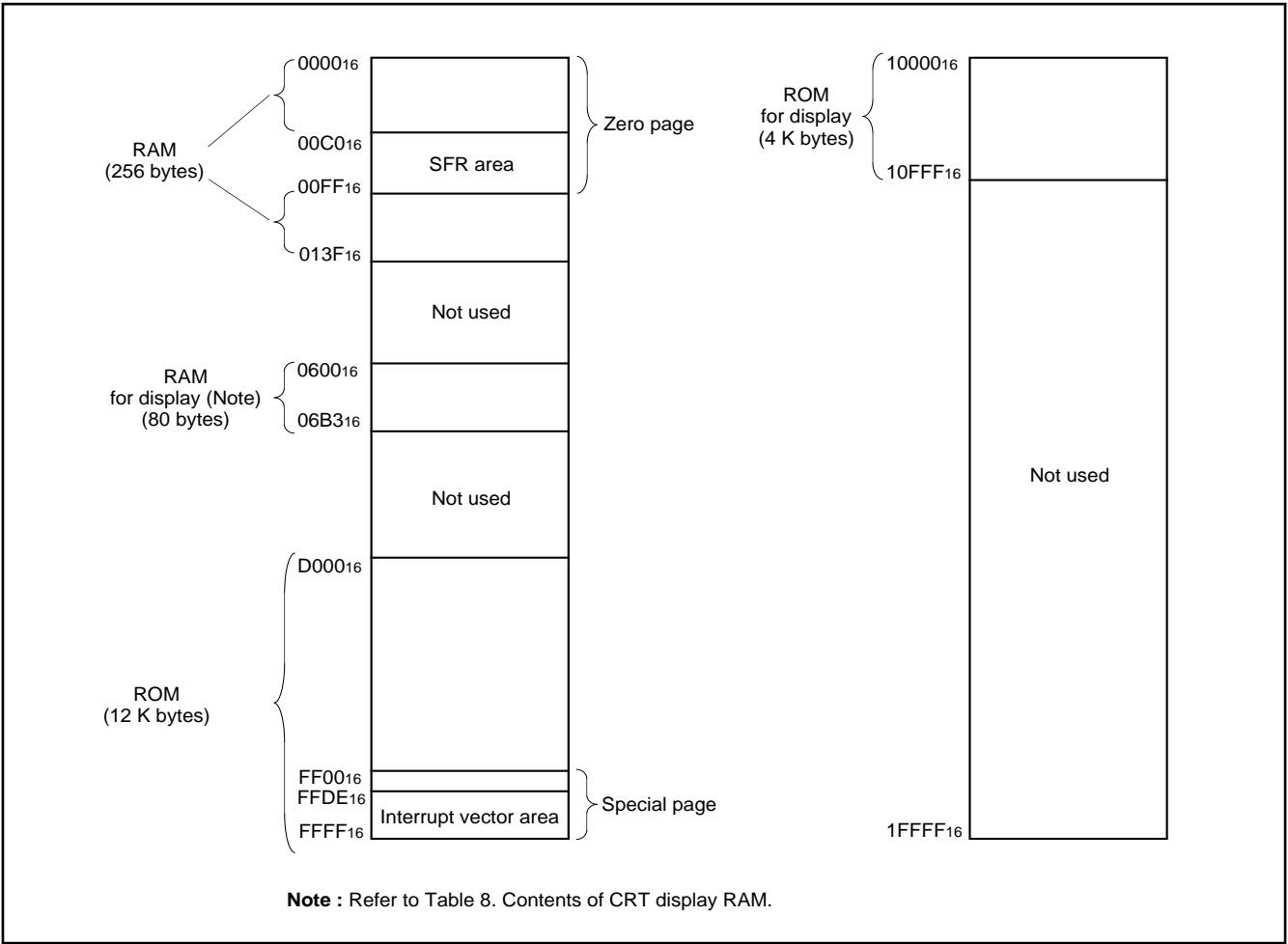
Fig. 2. Memory map
