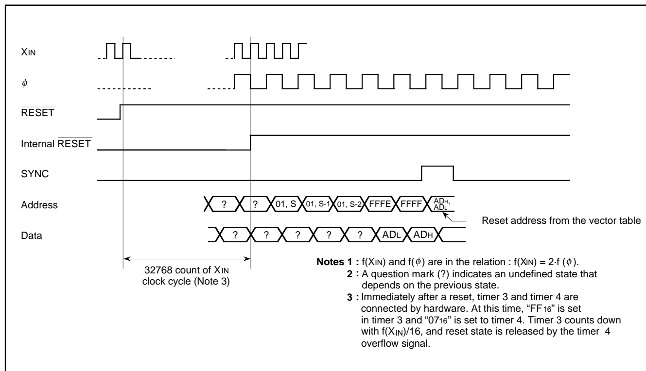
Fig. 53. Reset Sequence
