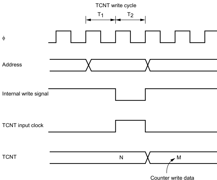
Figure 13-3 Contention between TCNT Write and Increment
