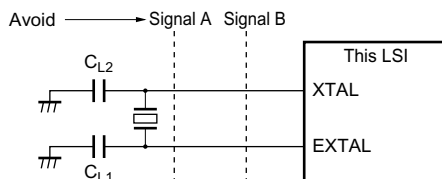
Figure 19-6 Note on Board Design of Oscillator Circuit
