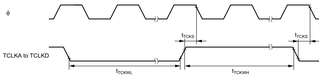
Figure 21-8 TPU Clock Input Timing
