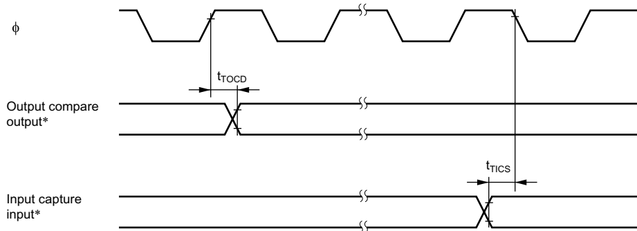
Figure 21-7 TPU Input/Output Timing
