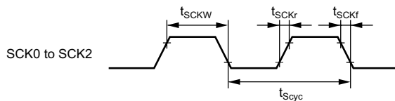
Figure 21-9 SCK Clock Input Timing
