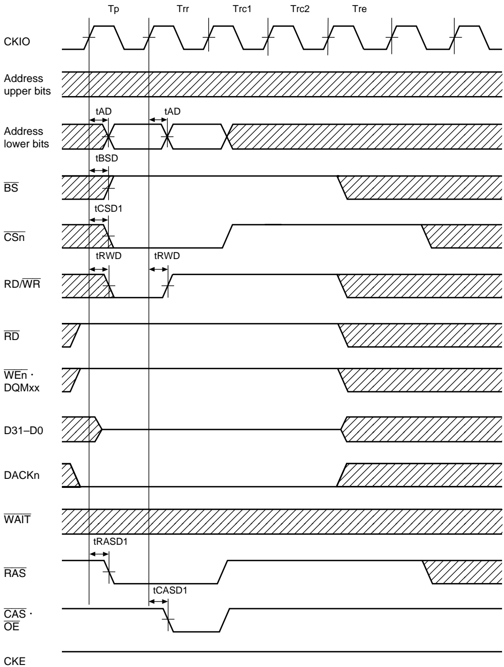
Figure 22.31 Synchronous DRAM Auto-Refresh Cycle (Shown from Precharge Cycle, TRP = 1 Cycle, TRAS = 4 Cycles)
