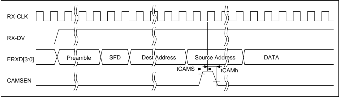
Figure 22.77 CAMSEN Input Timing
