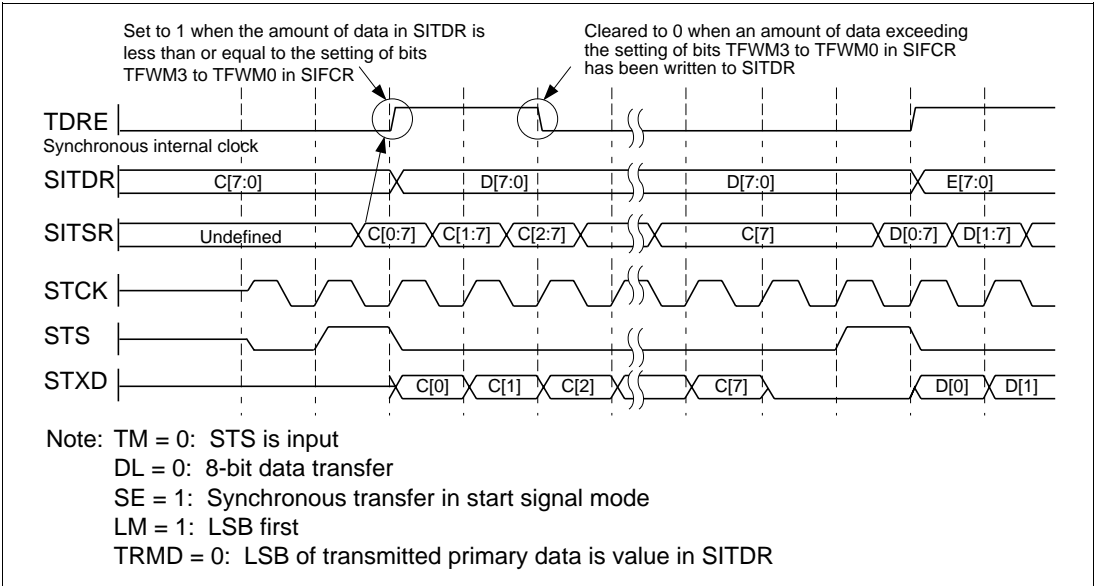
Figure 15.10 Transmission: Interval Transfer Mode (TM = 0 Mode)/LSB First
