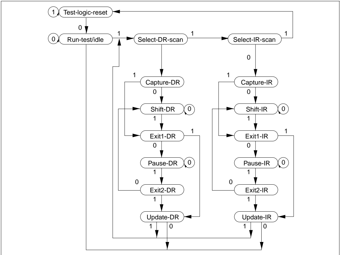
Figure 18.2 TAP Controller State Transitions
