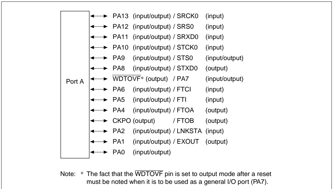
Figure 20.1 Port A
