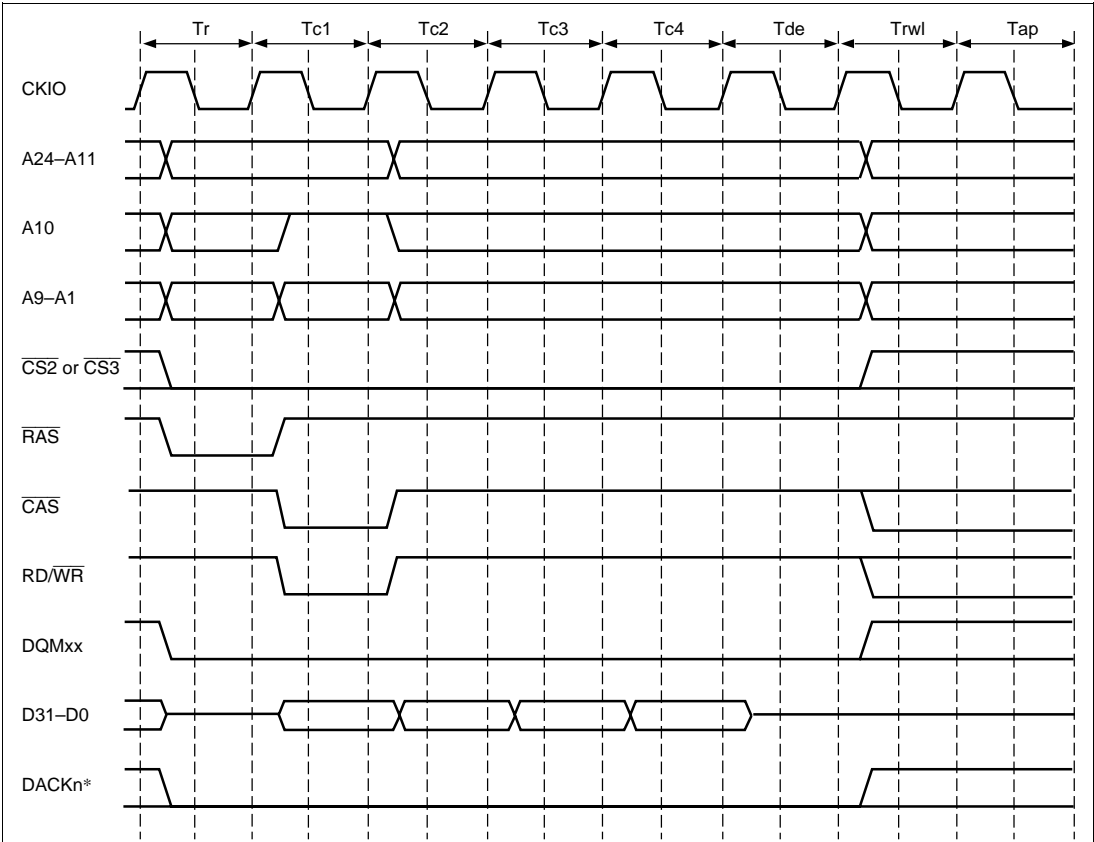
Figure 7.23 (b) Basic Burst Write Timing (Auto-Precharge) Iφ : Eφ = 1 : 1
