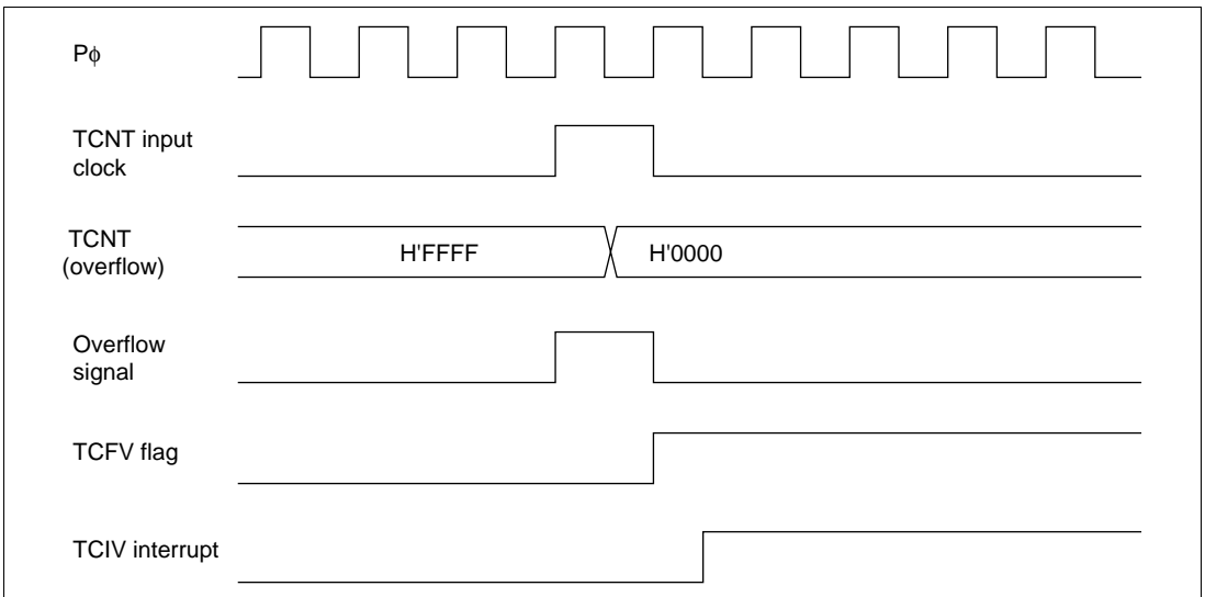
Figure 17.40 TCIV Interrupt Setting Timing
