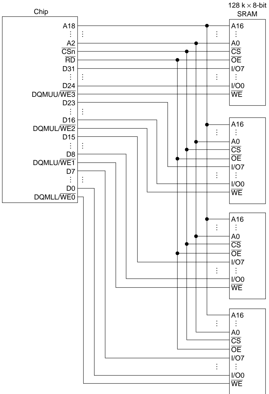
Figure 7.10 Example of 32-Bit Data Width SRAM Connection
