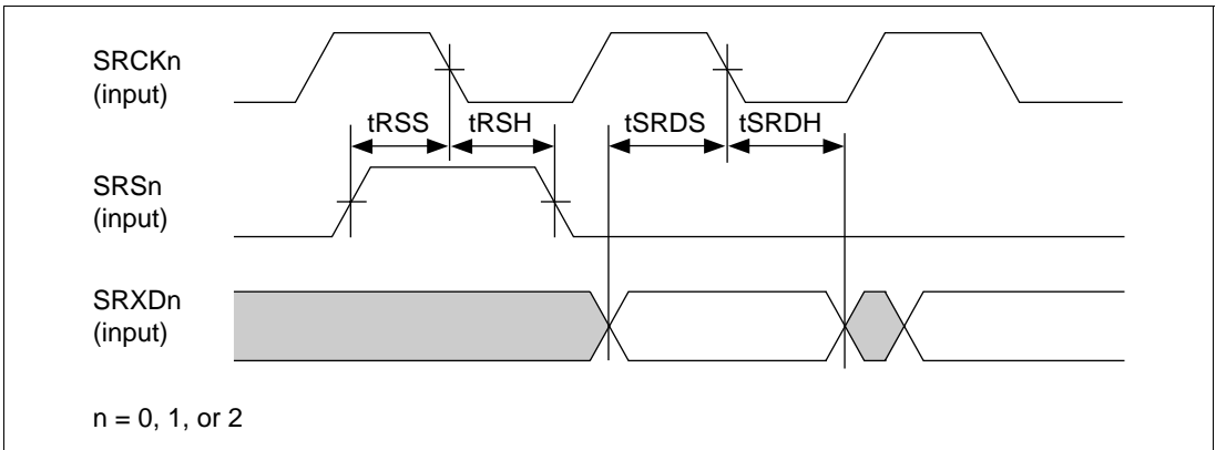
Figure 22.61 SIOF / SIO Receive Timing
