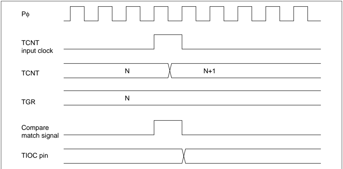
Figure 17.32 Output Compare Output Timing
