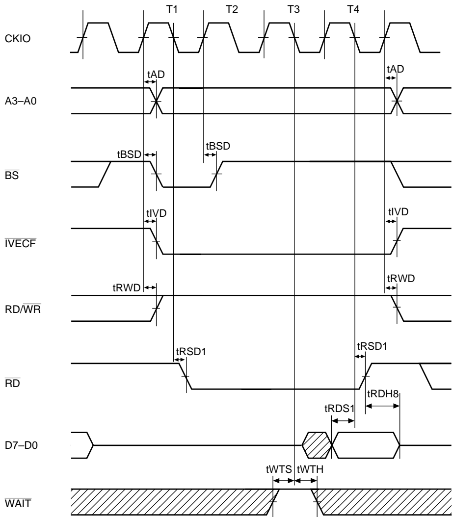
Figure 22.43 Interrupt Vector Fetch Cycle (No Wait, I\phi:E\phi = 1:1 )
