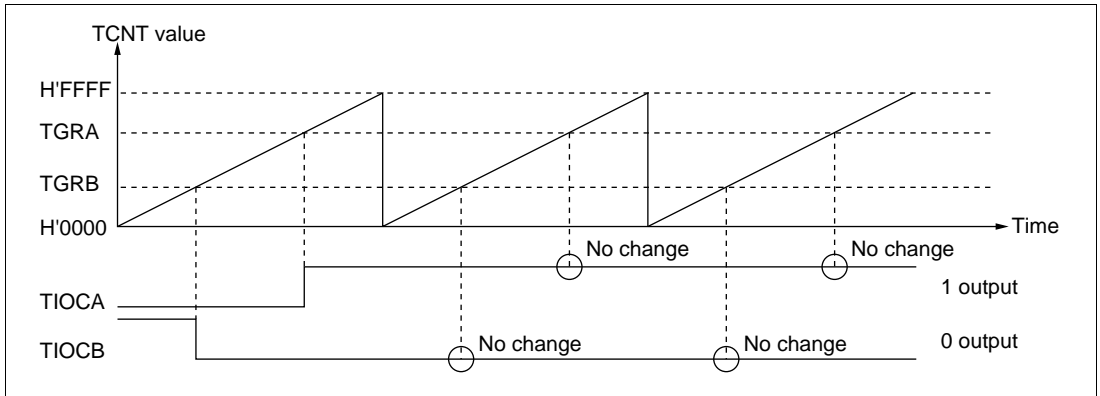
Figure 17.10 Example of 0 Output/1 Output Operation
