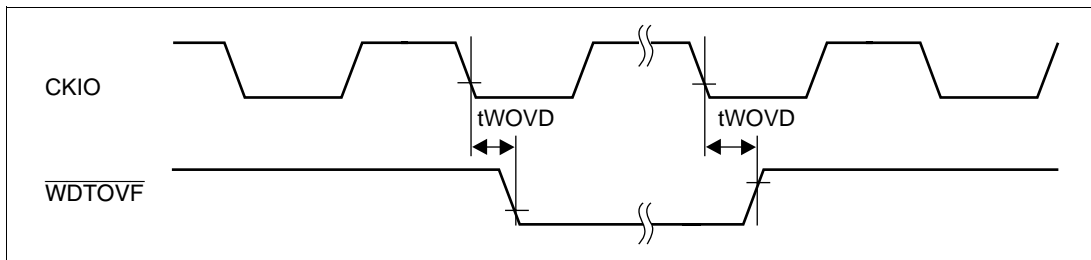
Figure 22.59 Watchdog Timer Output Timing ( t_{Ecy}:t_{Pcyc} other than 1:1)
