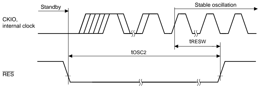
Figure 22.4 Power-On Oscillation Stabilization Time at Power-On
