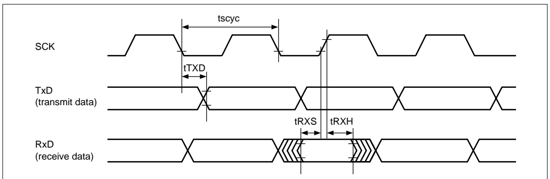
Figure 22.53 SCI Input/Output Timing (Synchronous Mode)
