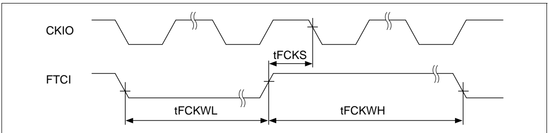
Figure 22.51 FRT Clock Input Timing ( t_{Ecyc}:t_{Pcyc} other than 1:1)
