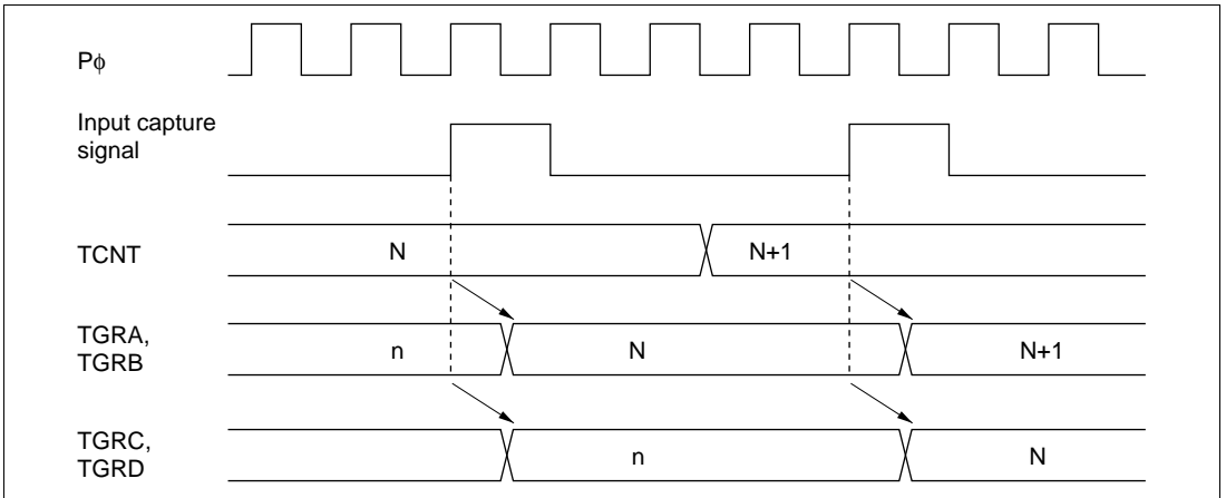
Figure 17.37 Buffer Operation Timing (Input Capture)
