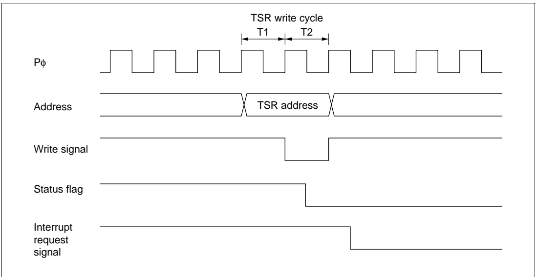
Figure 17.42 Timing for Status Flag Clearing by CPU
