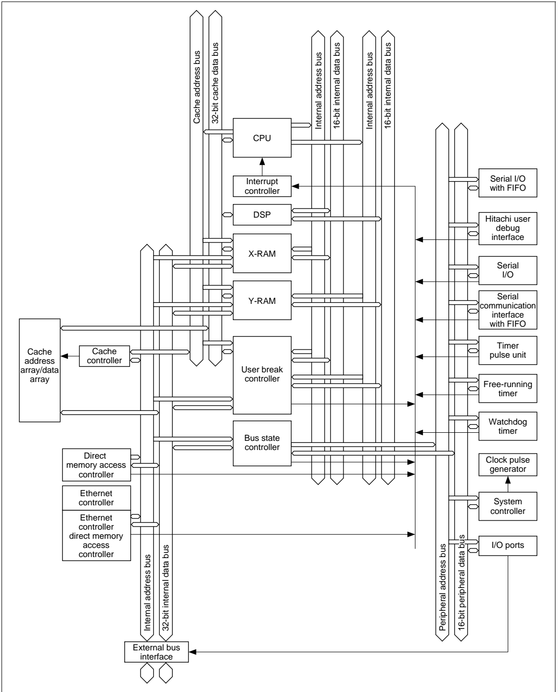
Figure 1.1 Block Diagram of SH7616
