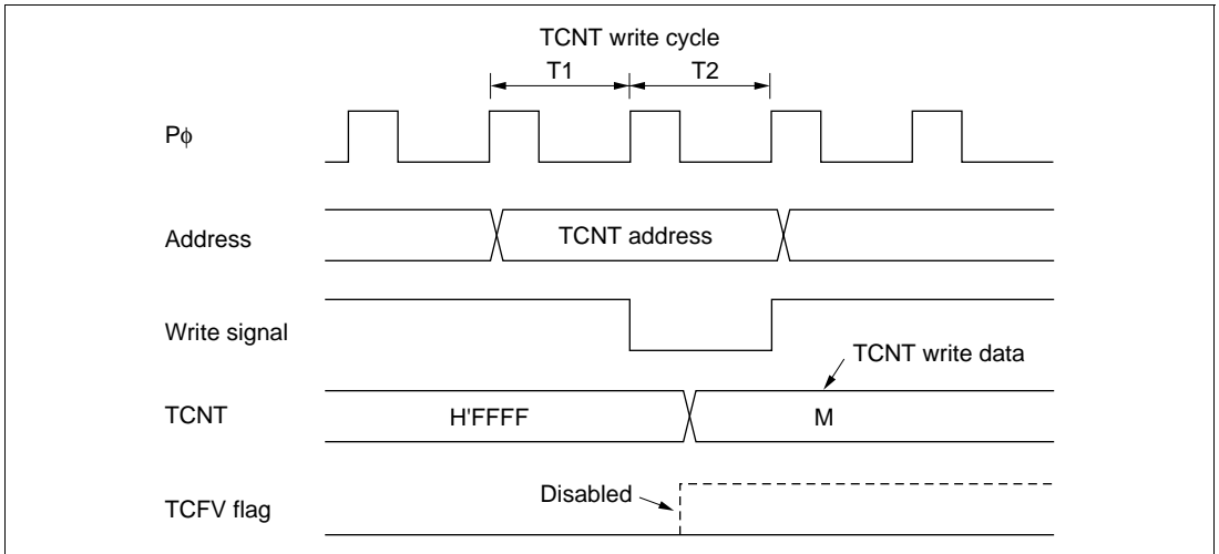
Figure 17.53 Contention between TCNT Write and Overflow
