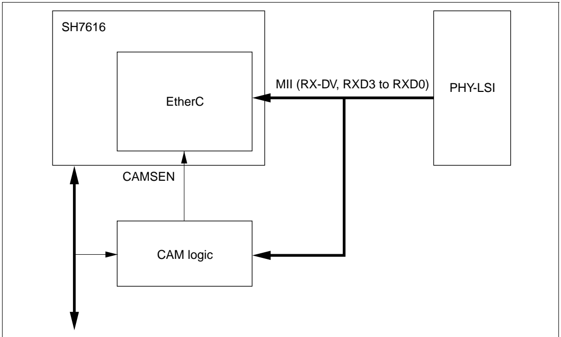
Figure 9.7 CAM Circuit Connection
