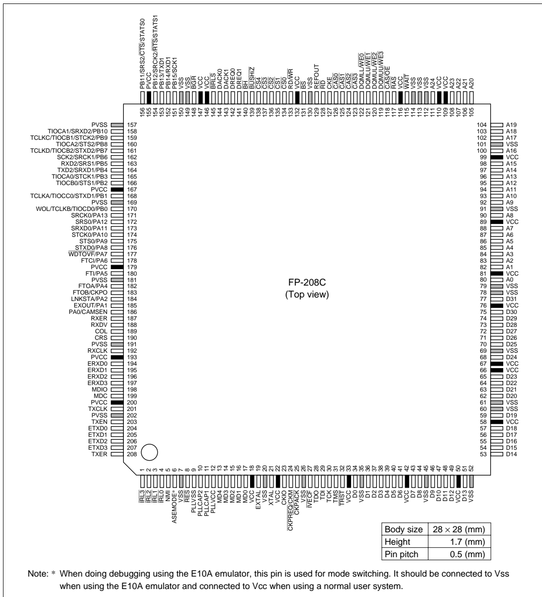
Figure 1.2 SH7616 Pin Arrangement (FP-208C)
