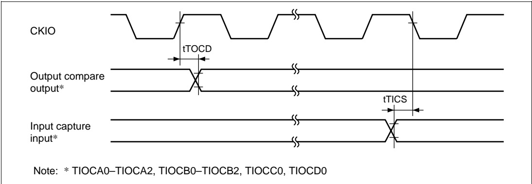
Figure 22.55 TPU Input/Output Timing ( t_{Ecyc}:t_{Pcyc} = 1:1 )
