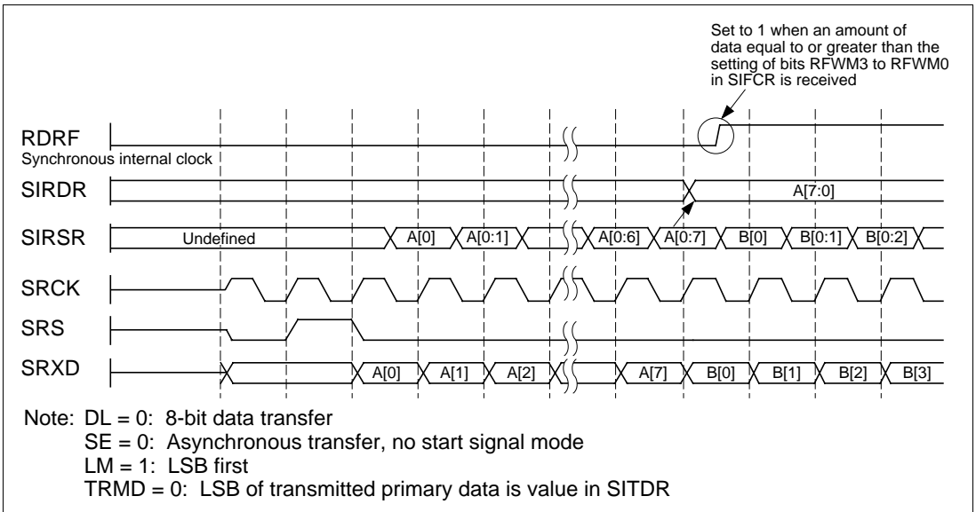
Figure 15.5 Reception: Continuous Transfer Mode/LSB First
