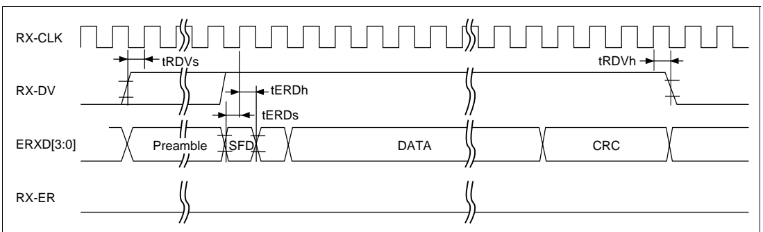
Figure 22.71 MII Receive Timing (Normal Operation)
