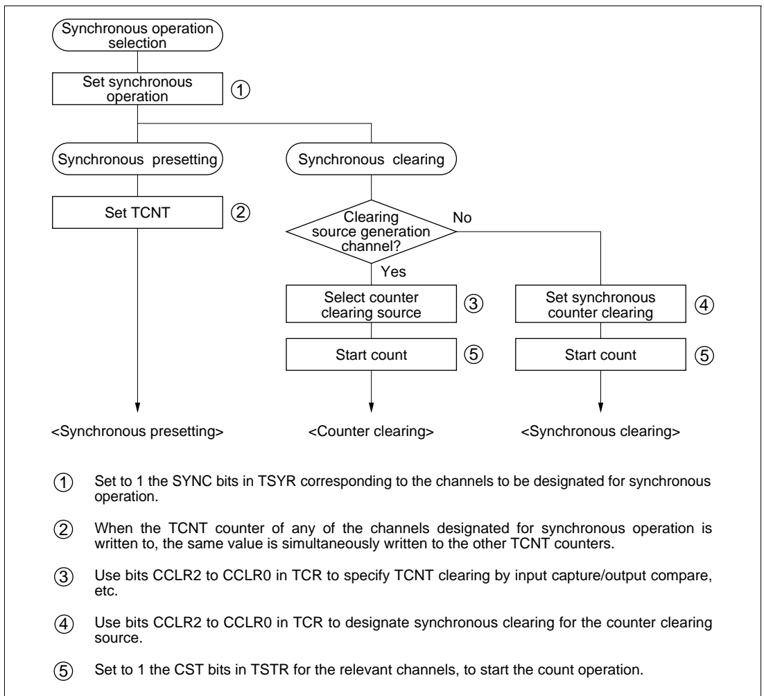
Figure 17.14 Example of Synchronous Operation Setting Procedure
