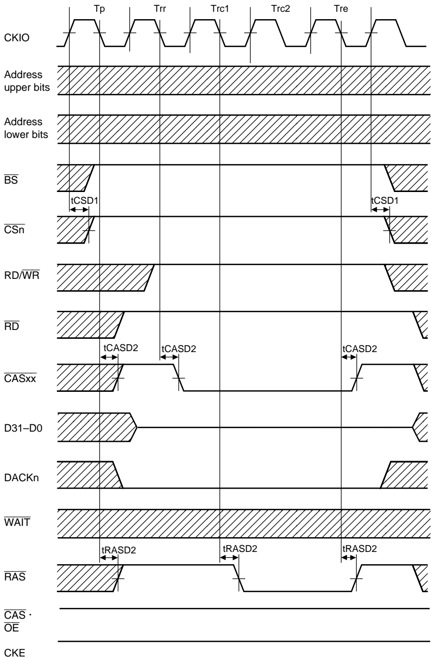
Figure 22.41 DRAM \overline{\text{CAS}} -Before- \overline{\text{RAS}} Refresh Cycle (TRP = 1 Cycle, TRAS = 2 Cycles)
