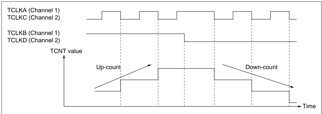
Figure 17.27 Example of Phase Counting Mode 2 Operation
