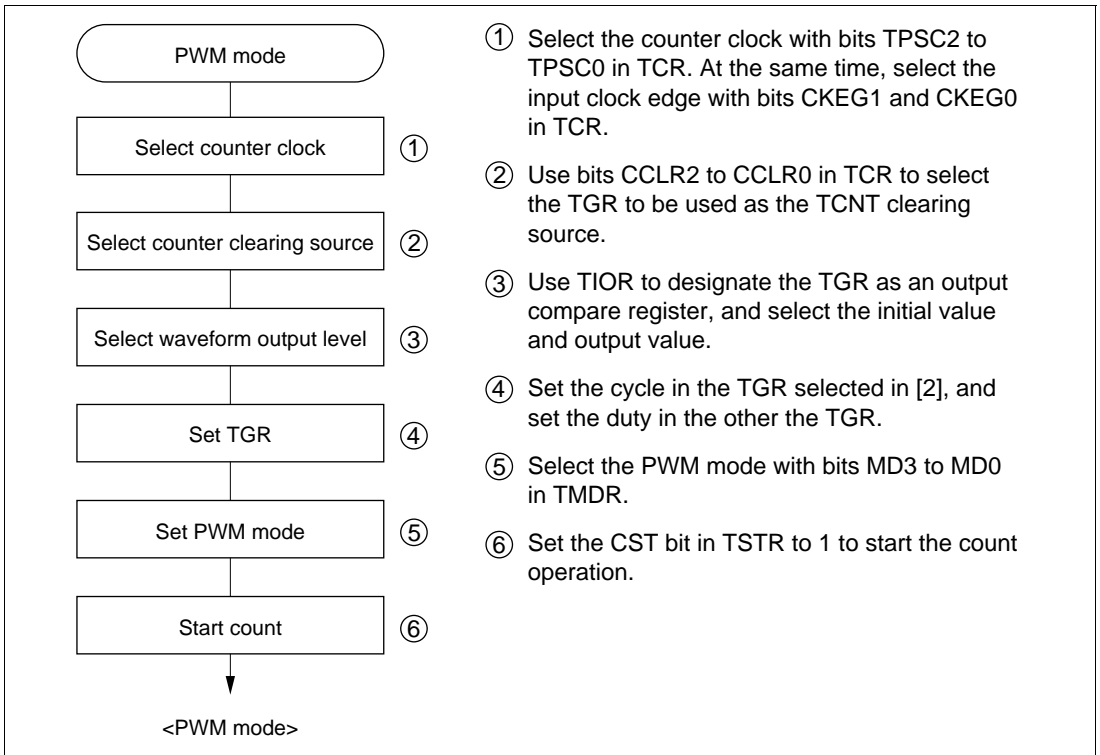
Figure 17.21 Example of PWM Mode Setting Procedure
