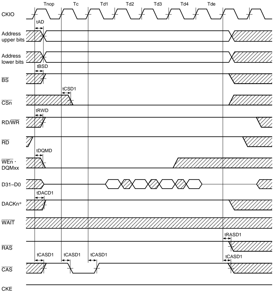
Figure 22.18 Synchronous DRAM Read Bus Cycle (Bank Active, Same Row Access, CAS Latency = 1 Cycle)
