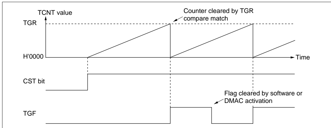
Figure 17.8 Periodic Counter Operation
