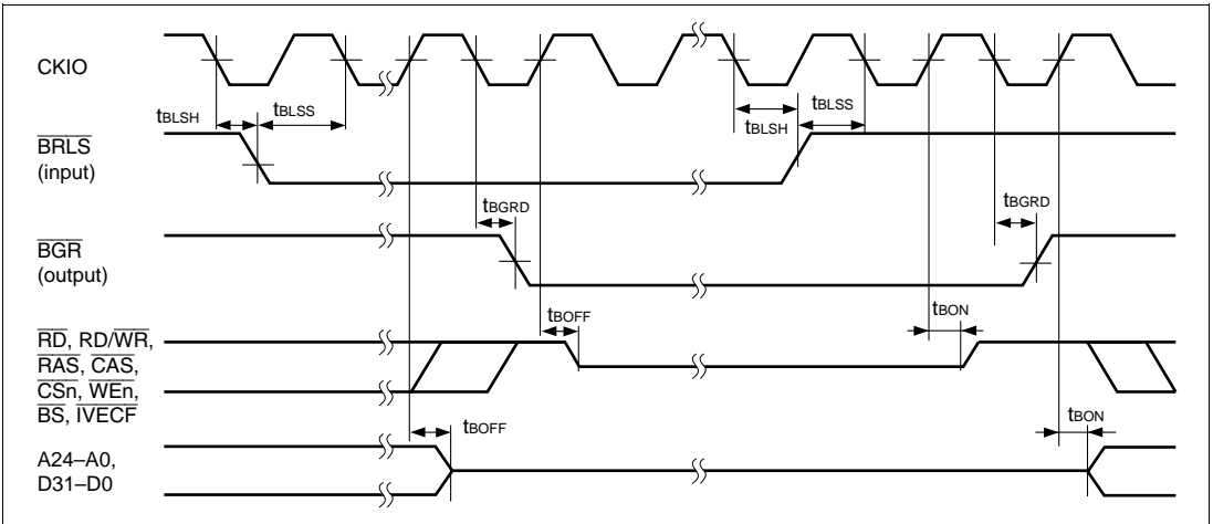
Figure 22.10 Bus Release Timing
