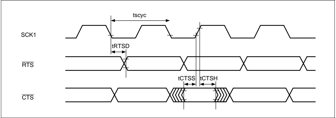
Figure 22.54 \overline{\text{RTS}} and \overline{\text{CTS}} Input/Output Timing
