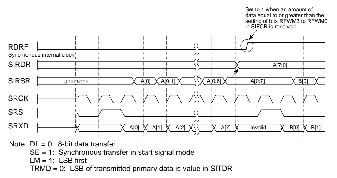
Figure 15.4 Reception: Interval Transfer Mode/LSB First
