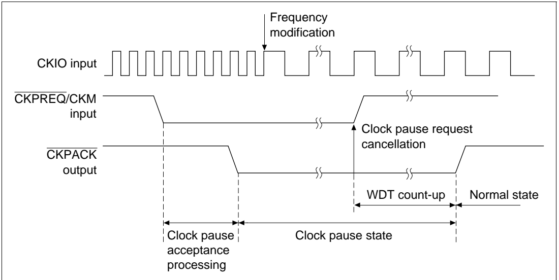
Figure 21.2 Clock Pause Function Timing Chart (PLL Circuit 1 Operating)
