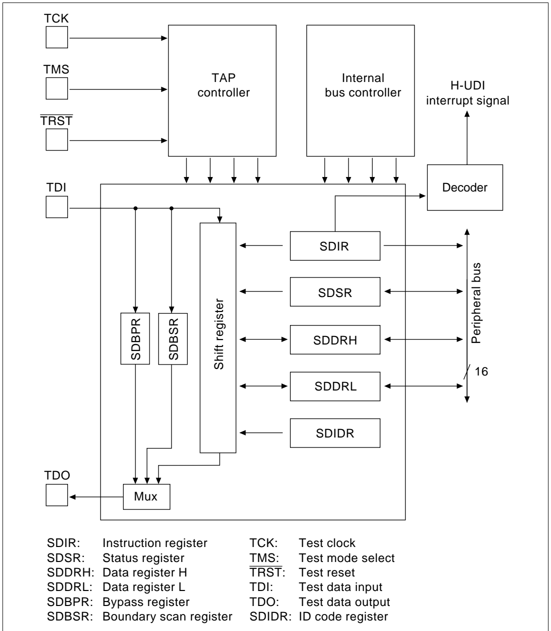
Figure 18.1 H-UDI Block Diagram
