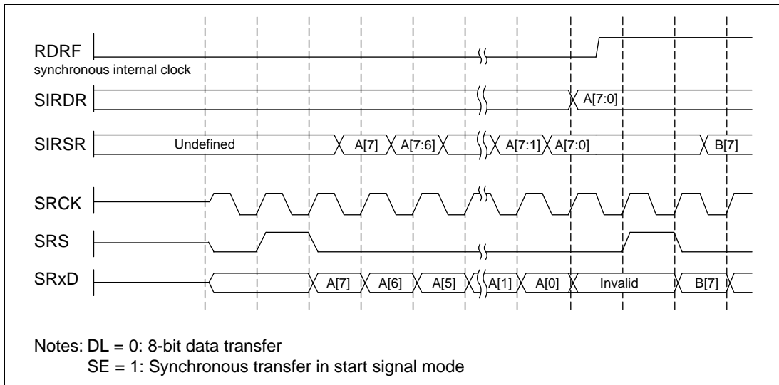
Figure 16.2 Reception: Interval Transfer Mode
