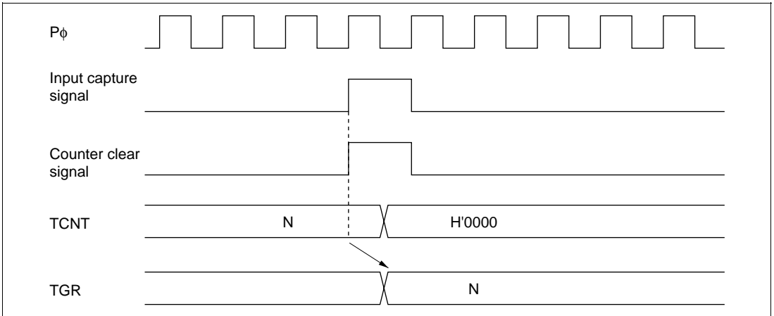
Figure 17.35 Counter Clear Timing (Input Capture)
