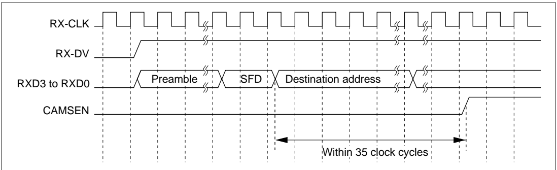
Figure 9.8 CAM Signal Timing
