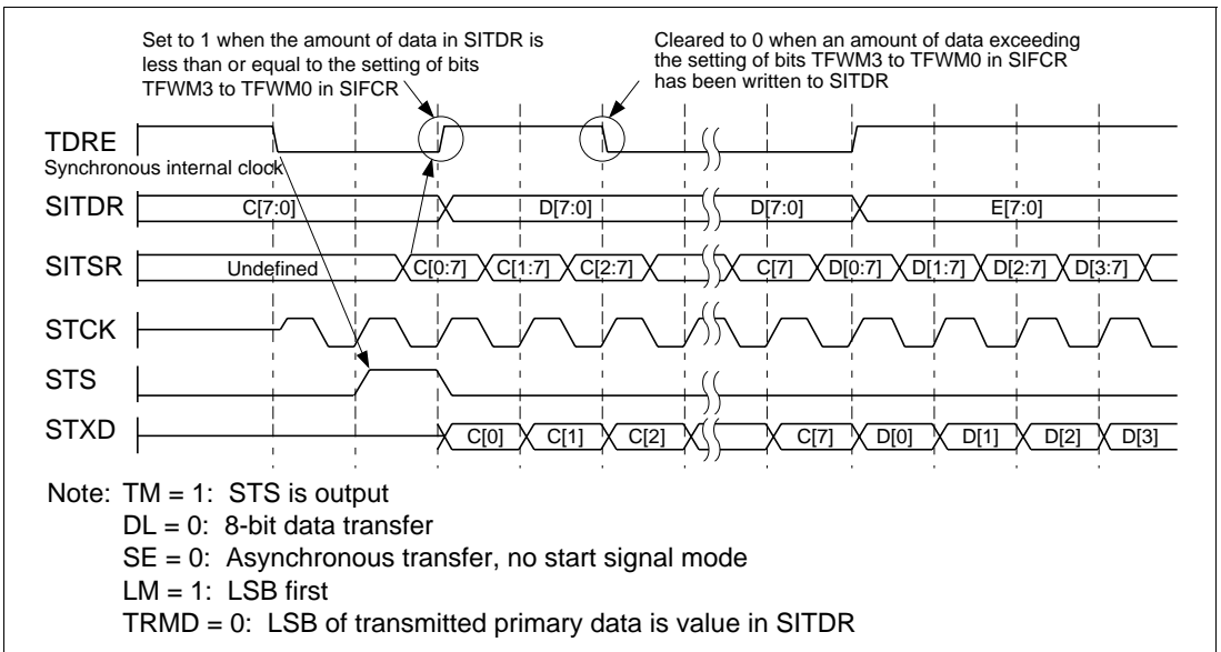
Figure 15.13 Transmission: Continuous Transfer Mode (TM = 1 Mode)/LSB First
