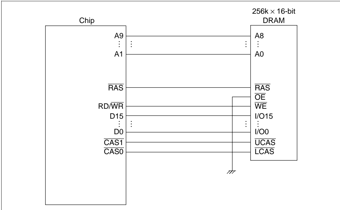
Figure 7.36 Example of DRAM Connection (16-Bit Data Width)
