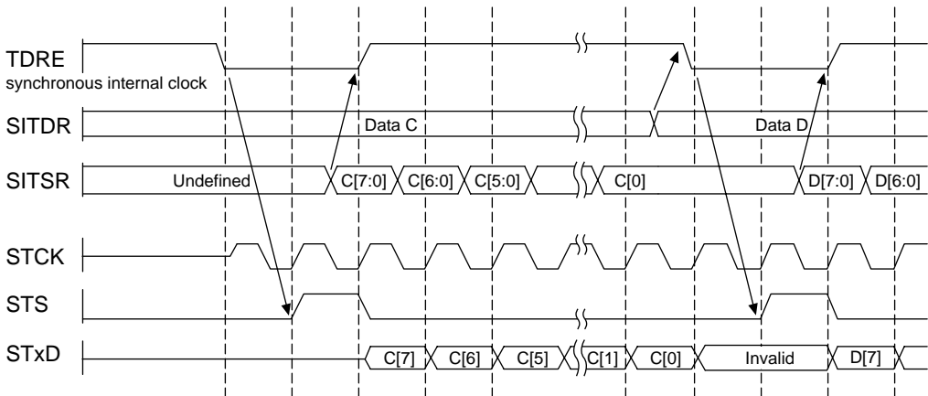
Figure 16.5 Transmission: Continuous Transfer Mode (TM = 0 Mode)
