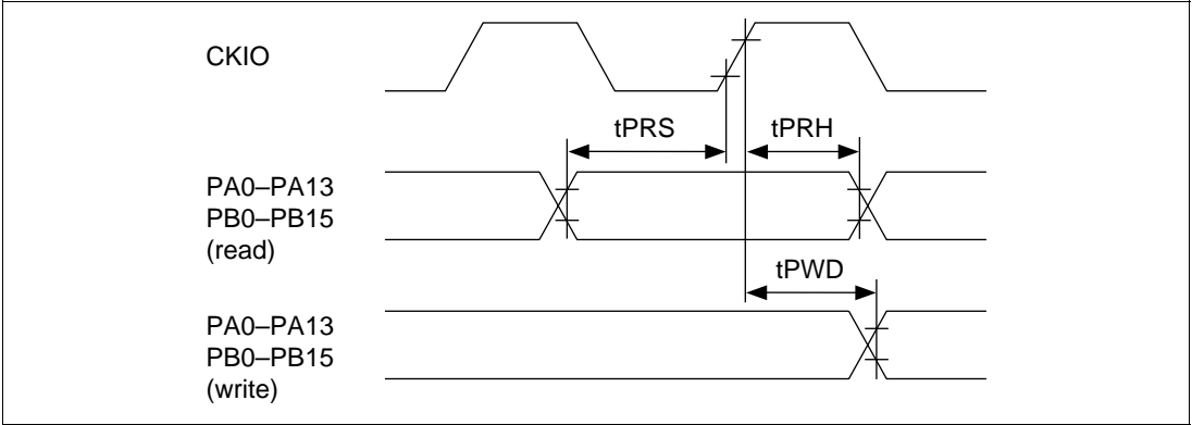
Figure 22.67 I/O Port Input/Output Timing ( t_{EcyC}:t_{PcyC} = 1:1 )
