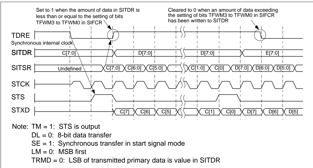
Figure 15.8 Transmission: Interval Transfer Mode (TM = 1 Mode)/MSB First
