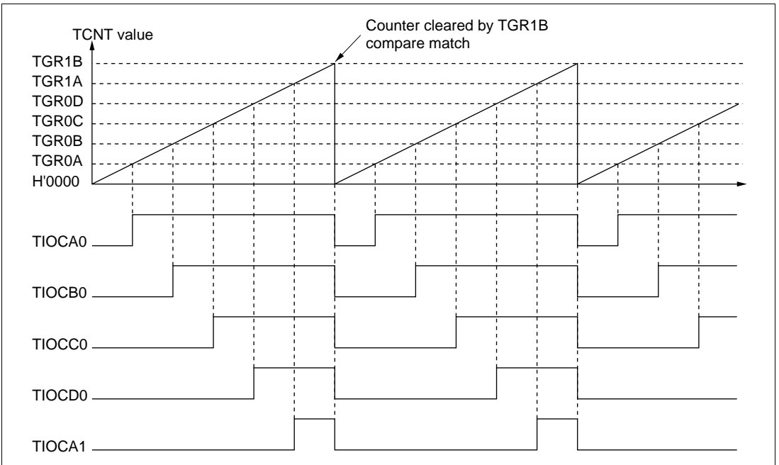
Figure 17.23 Example of PWM Mode Operation (2)
