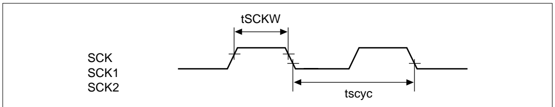
Figure 22.52 Input Clock Input/Output Timing
