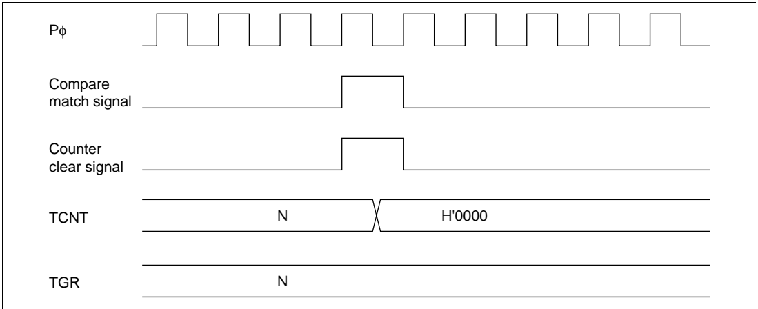
Figure 17.34 Counter Clear Timing (Compare Match)
