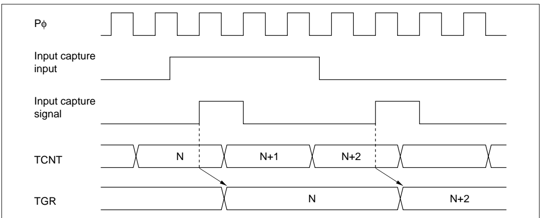
Figure 17.33 Input Capture Input Signal Timing
