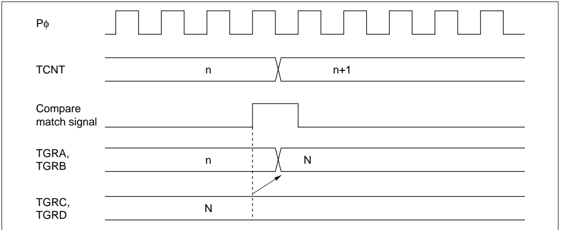
Figure 17.36 Buffer Operation Timing (Compare Match)
