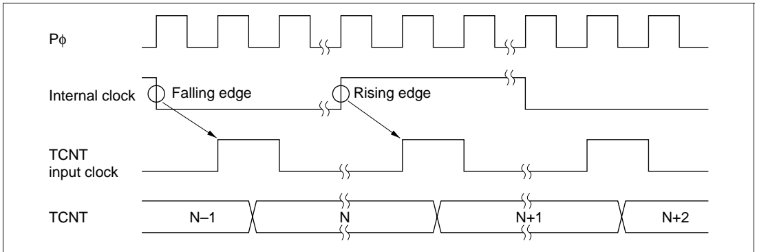
Figure 17.30 Count Timing in Internal Clock Operation
