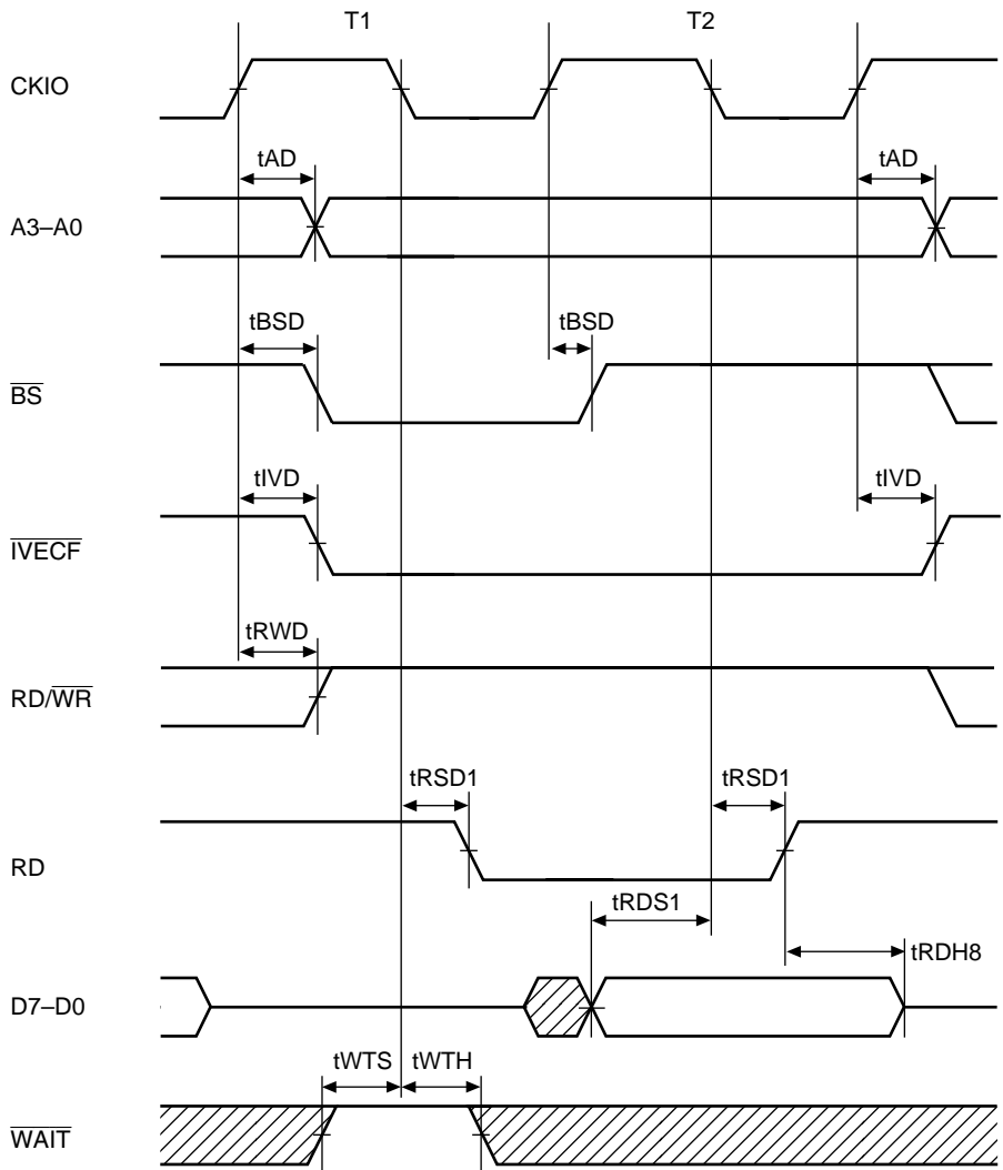
Figure 22.44 Interrupt Vector Fetch Cycle (No Wait, I \phi :E \phi other than 1:1)
