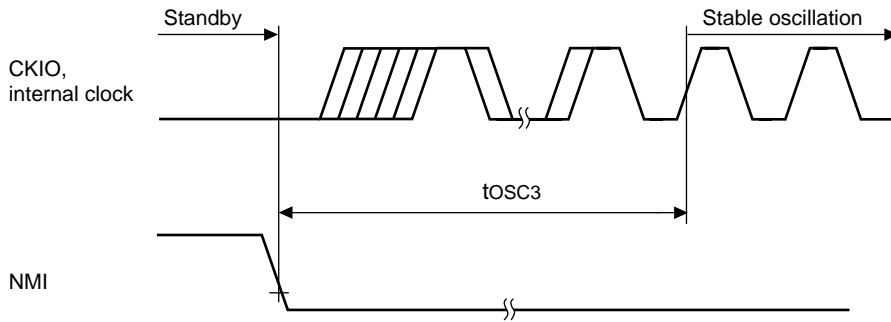
Figure 22.6 Oscillation Stabilization Time after Standby Recovery (Recovery by NMI)
