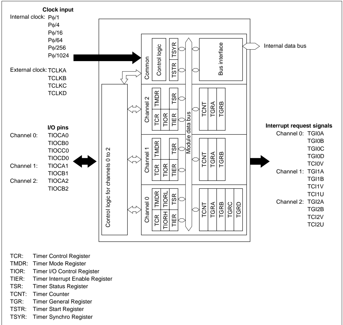
Figure 17.1 TPU Block Diagram
