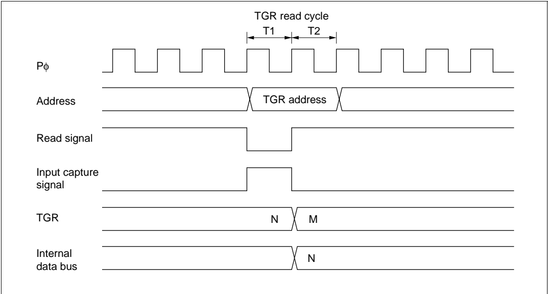
Figure 17.49 Contention between TGR Read and Input Capture
