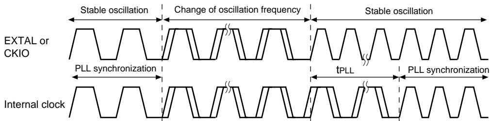
Figure 22.7 PLL Synchronization Stabilization Time
