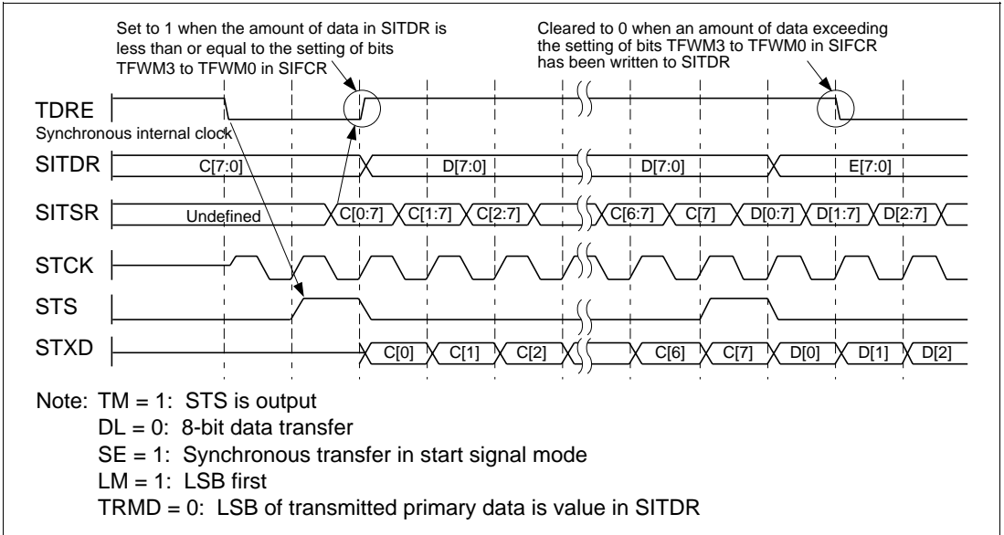
Figure 15.12 Transmission: Interval Transfer Mode (TM = 1 Mode)/LSB First
