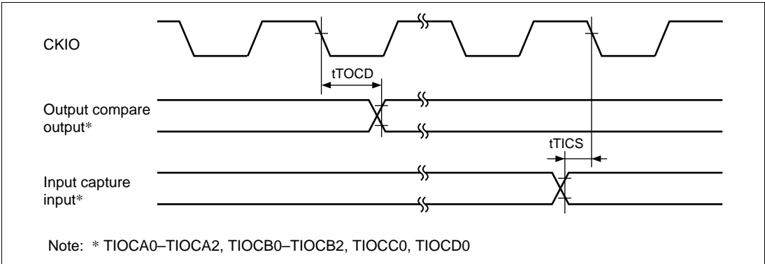
Figure 22.56 TPU Input/Output Timing ( t_{Ecyc}:t_{Pcyc} other than 1:1)
