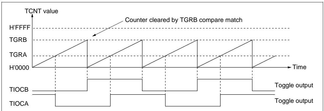
Figure 17.11 Example of Toggle Output Operation
