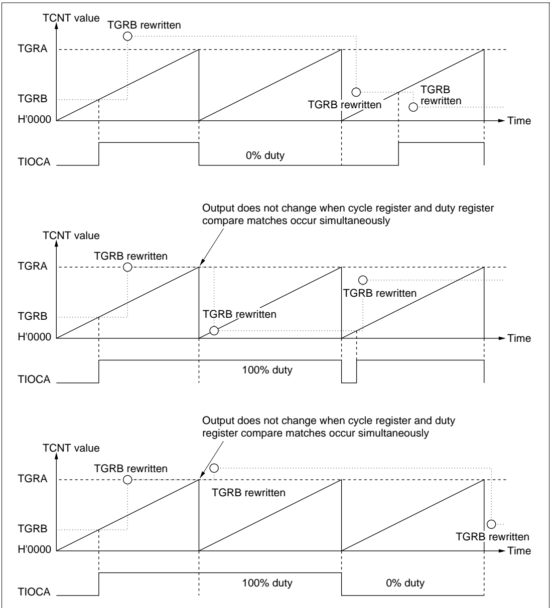
Figure 17.24 Example of PWM Mode Operation (3)
