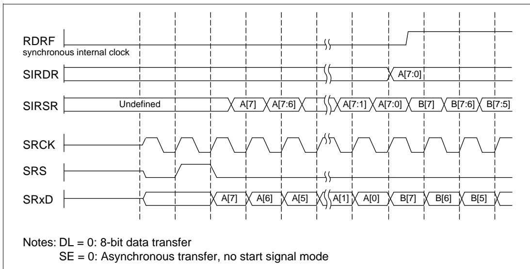
Figure 16.3 Reception: Continuous Transfer Mode
