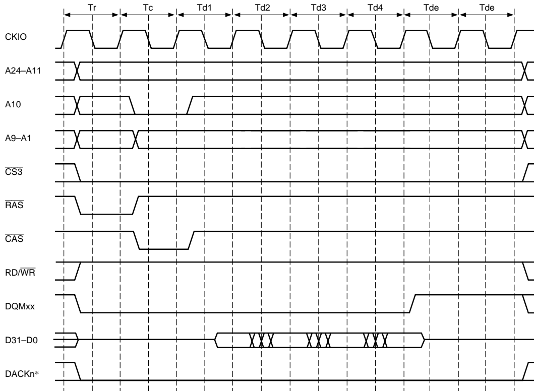
Figure 7.24 (b) Burst Read Timing (No Precharge) I\phi : E\phi = 1 : 1
