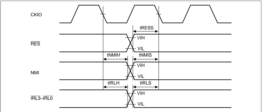
Figure 22.9 Interrupt Signal Input Timing
