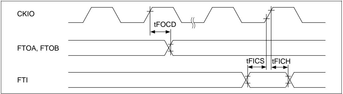
Figure 22.48 FRT Input/Output Timing ( t_{Ecyc}:t_{Pcyc} = 1:1 )
