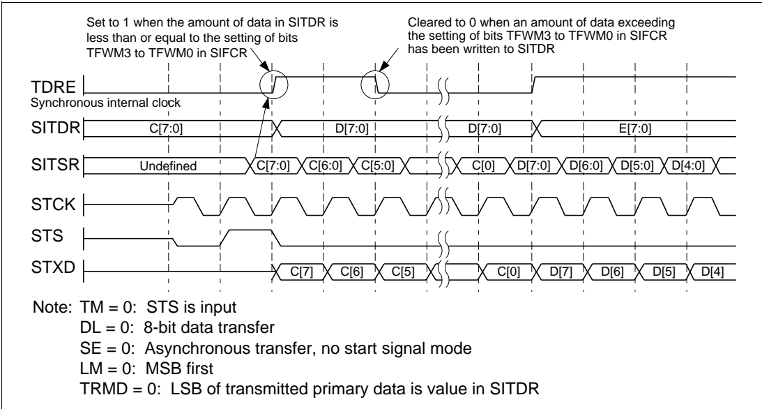
Figure 15.7 Transmission: Continuous Transfer Mode (TM = 0 Mode)/MSB First
