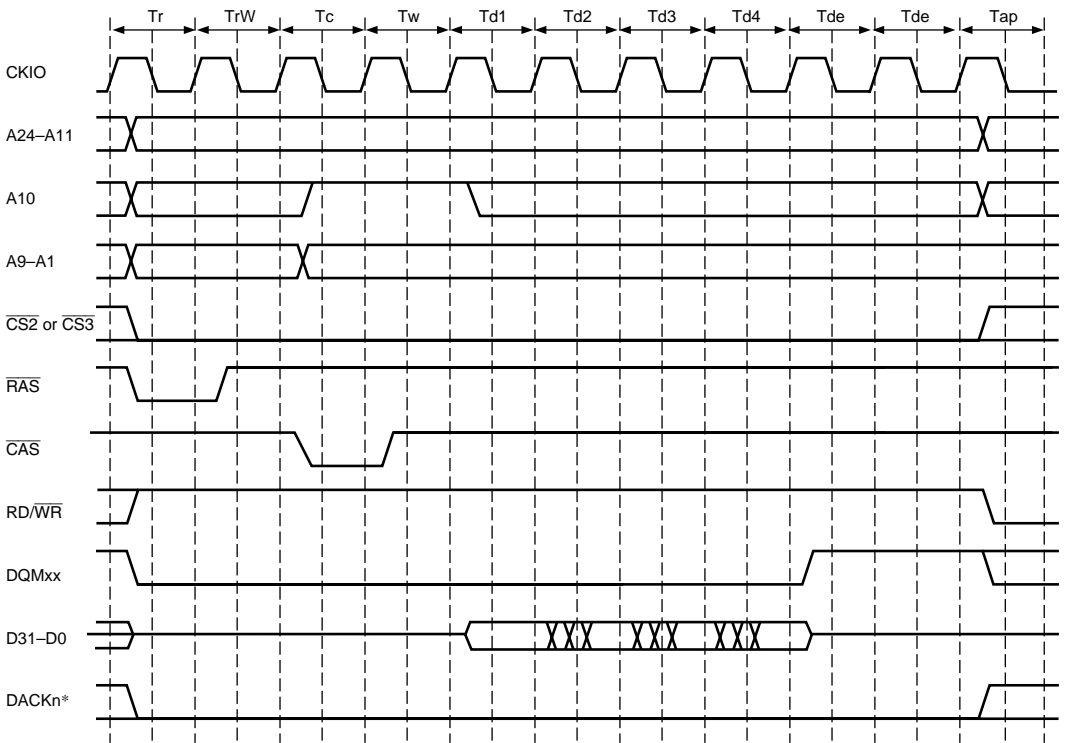
Figure 7.20 (b) Burst Read Wait Specification Timing (Auto-Precharge) I\phi : E\phi = 1 : 1
