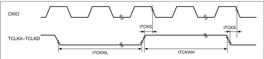
Figure 22.57 TPU Clock Input Timing
