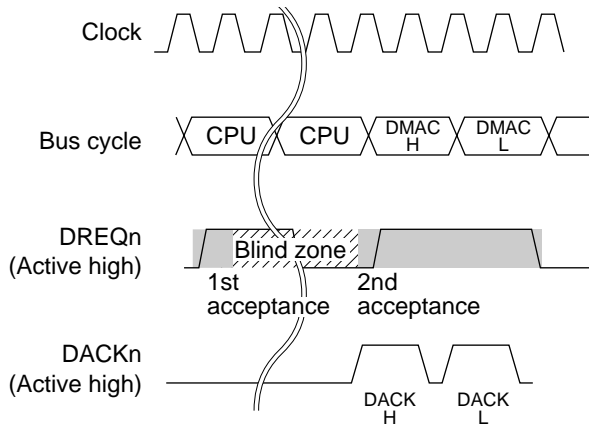
Figure 11.35 When a 16-Bit External Device is Connected (Edge Detection)
