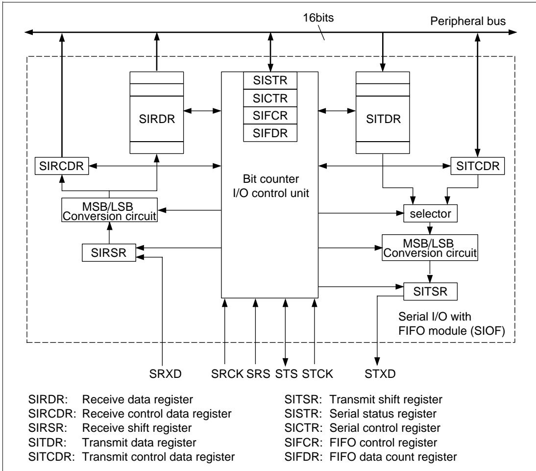
Figure 15.1 SIOF Block Diagram
