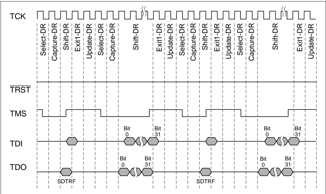
Figure 18.5 Data Input/Output Timing Chart (3)
