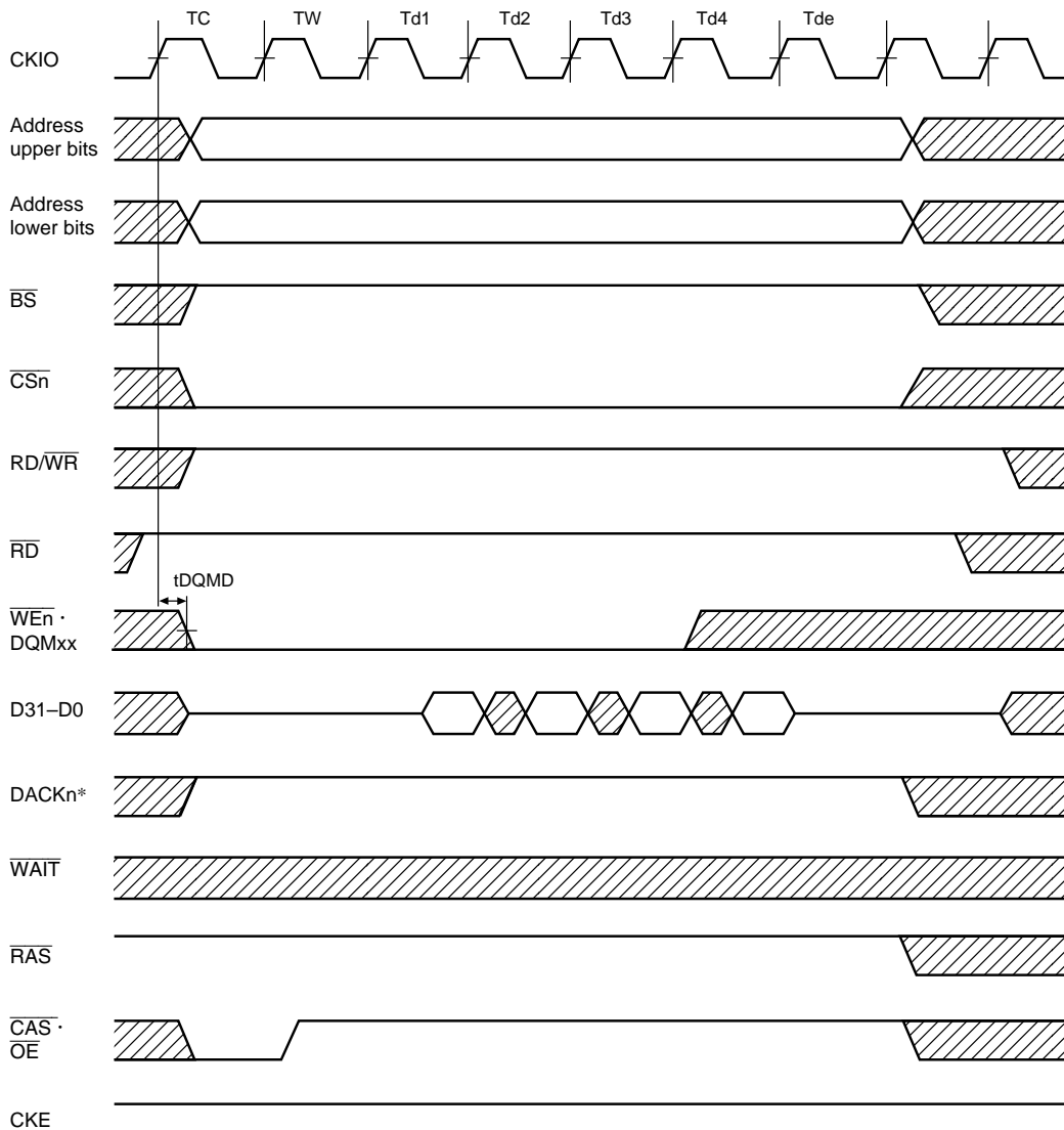
Figure 22.19 Synchronous DRAM Read Bus Cycle (Bank Active, Same Row Access, CAS Latency = 2 Cycles)
