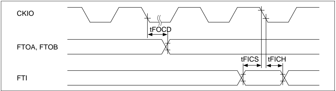
Figure 22.49 FRT Input/Output Timing ( t_{Ecyc}:t_{Pcyc} other than 1:1)
