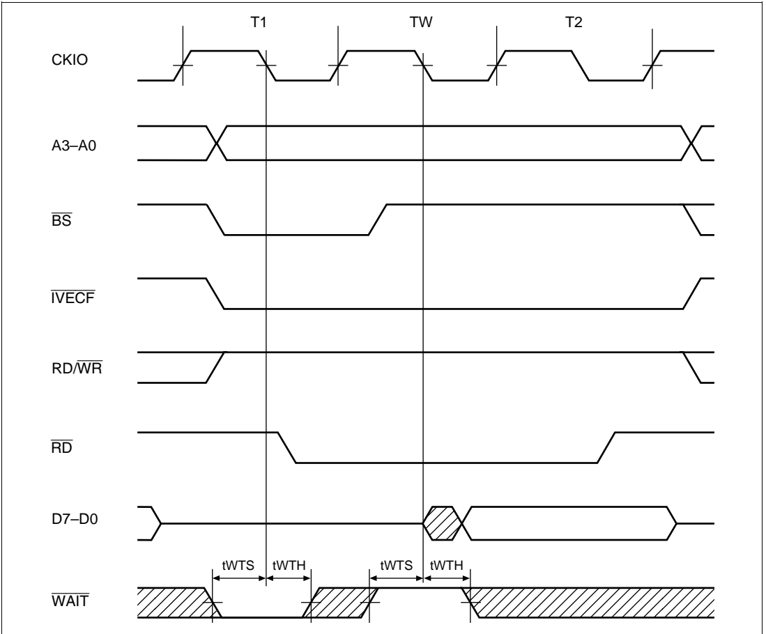
Figure 22.45 Interrupt Vector Fetch Cycle (External Wait Input, I\phi:E\phi other than 1:1)
