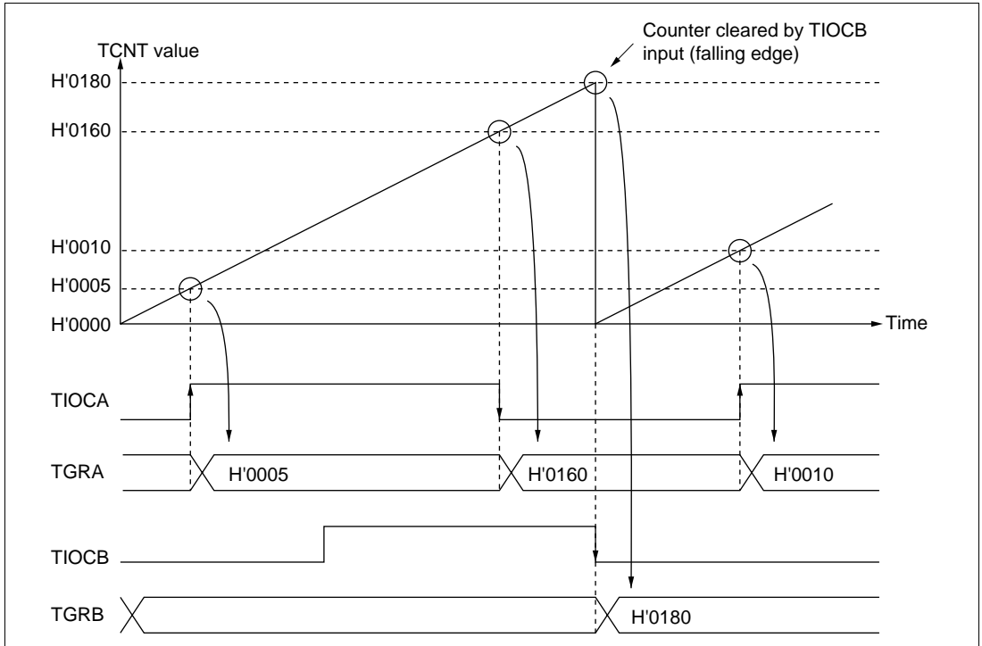
Figure 17.13 Example of Input Capture Operation
