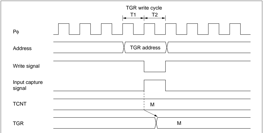
Figure 17.50 Contention between TGR Write and Input Capture
