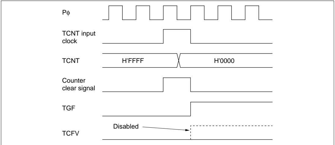
Figure 17.52 Contention between Overflow and Counter Clearing
