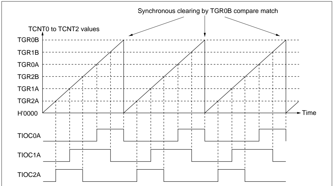
Figure 17.15 Example of Synchronous Operation
