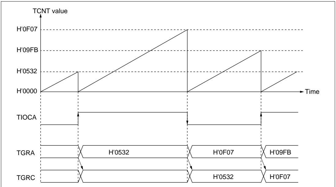
Figure 17.20 Example of Buffer Operation (2)
