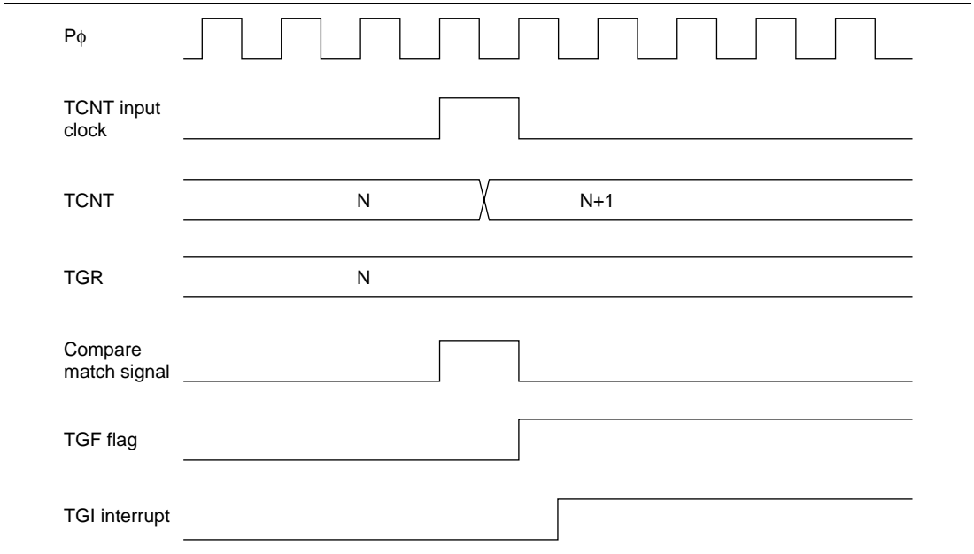
Figure 17.38 TGI Interrupt Timing (Compare Match)
