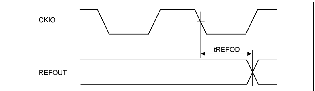
Figure 22.46 REFOUT Delay Time
