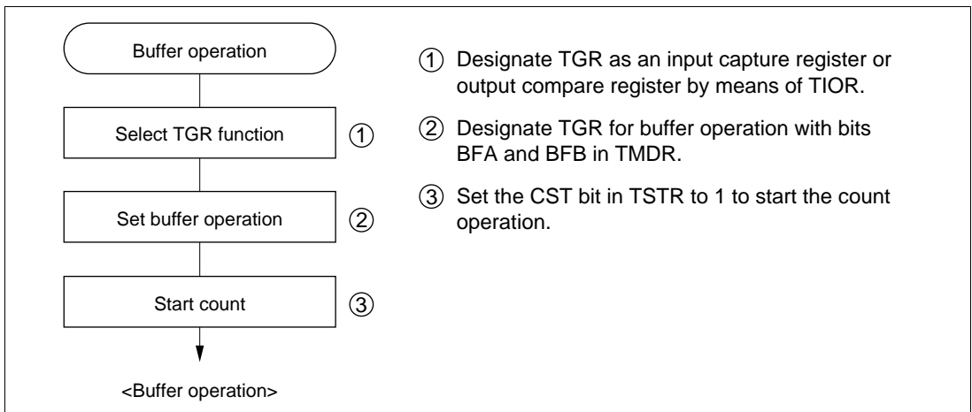
Figure 17.18 Example of Buffer Operation Setting Procedure
