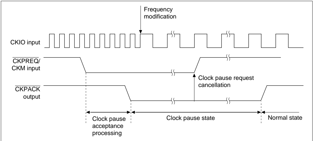
Figure 21.3 Clock Pause Function Timing Chart (PLL Circuit 1 Halted)
