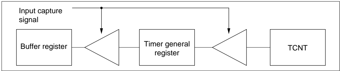
Figure 17.17 Input Capture Buffer Operation
