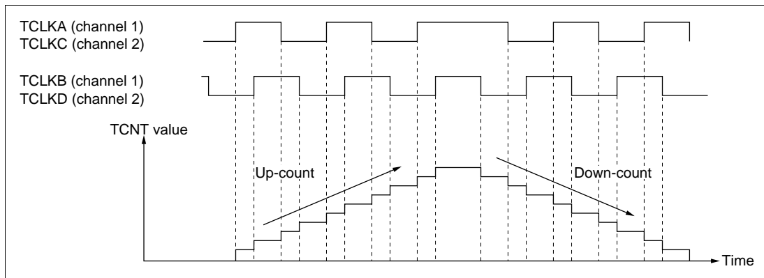
Figure 17.26 Example of Phase Counting Mode 1 Operation
