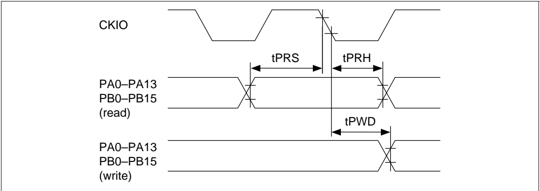
Figure 22.68 I/O Port Input/Output Timing ( t_{EcyC}:t_{PcyC} \neq 1:1 )
