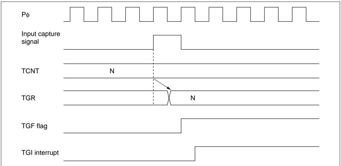
Figure 17.39 TGI Interrupt Timing (Input Capture)
