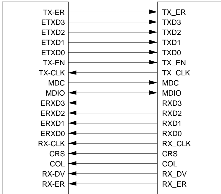
Figure 9.10 Example of Connection to DP83843
