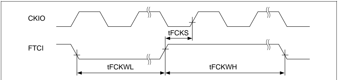
Figure 22.50 FRT Clock Input Timing ( t_{Ecyc}:t_{Pcyc} = 1:1 )
