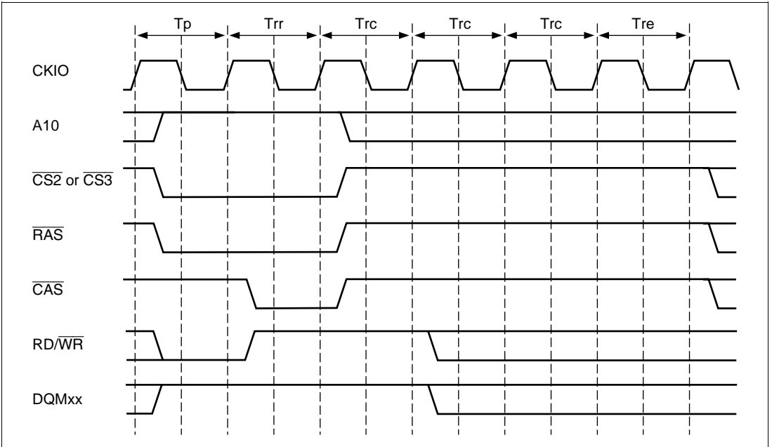
Figure 7.30 Auto-Refresh Timing
