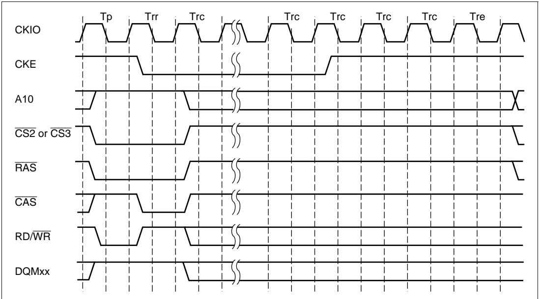
Figure 7.31 Self-Refresh Timing
