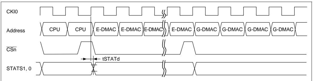
Figure 22.78 STATS Output Timing
