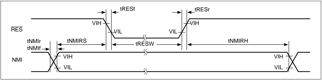
Figure 22.8 Reset Input Timing
