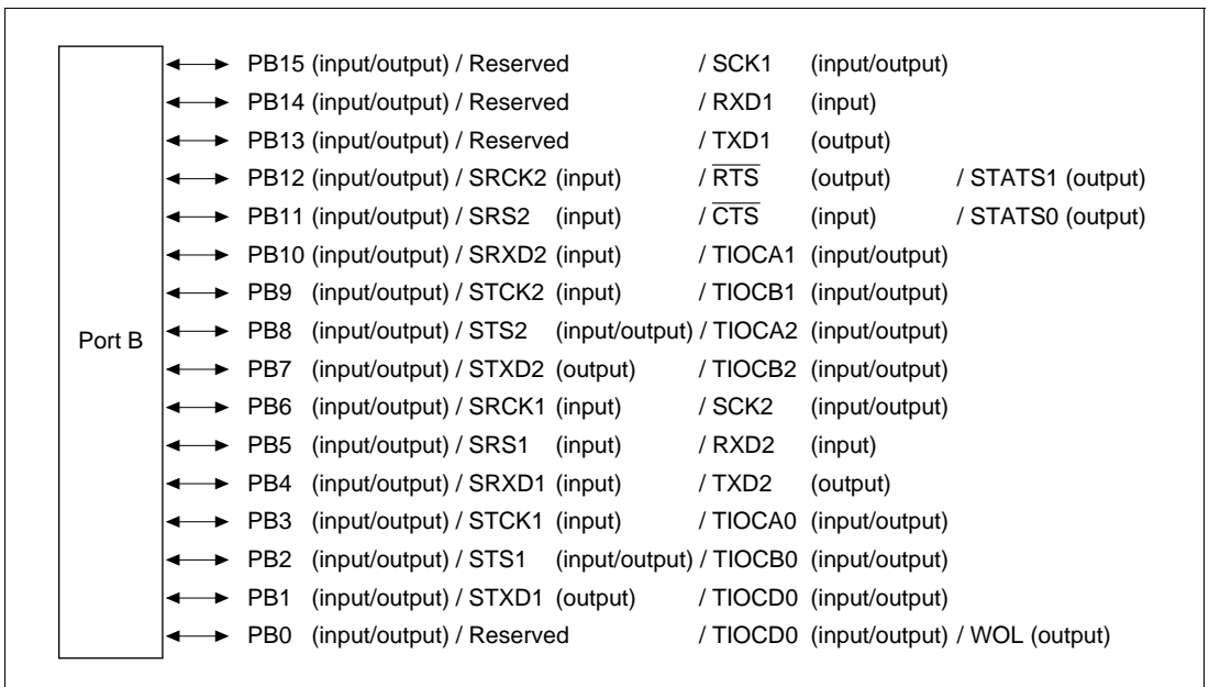
Figure 20.2 Port B
