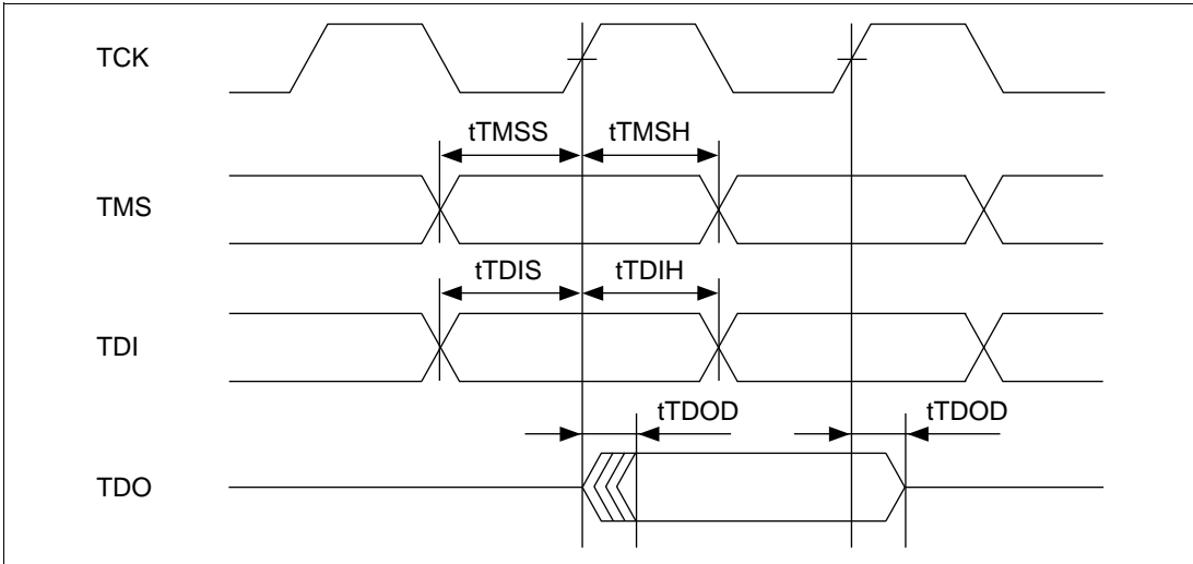
Figure 22.66 H-UDI Input/Output Timing
