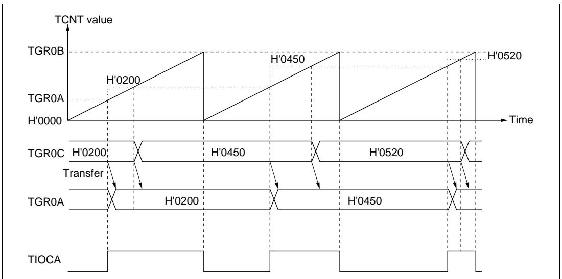
Figure 17.19 Example of Buffer Operation (1)
