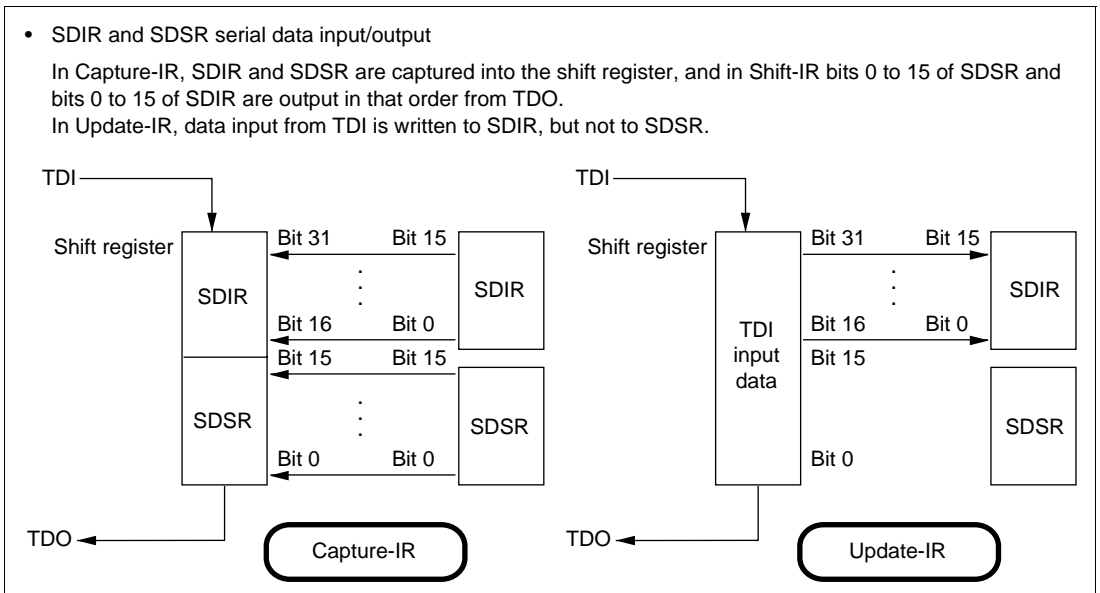
Figure 18.6 Serial Data Input/Output (1)
