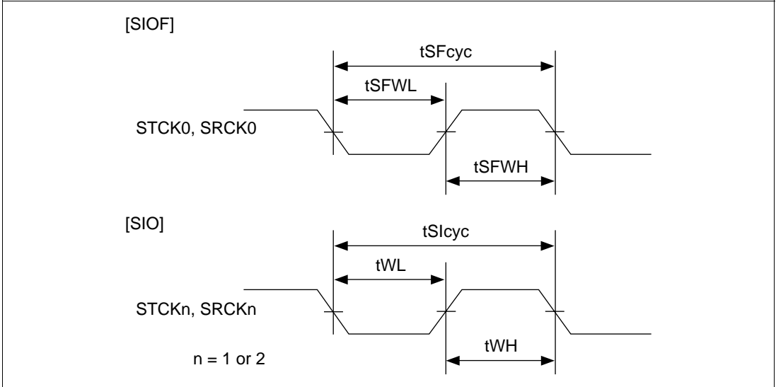
Figure 22.60 SIOF / SIO Input Clock Timing
