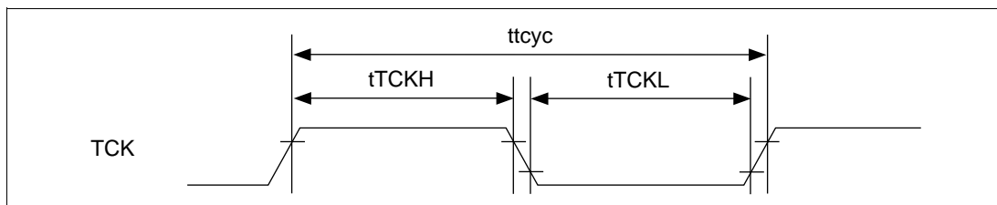
Figure 22.64 H-UDI Clock Timing
