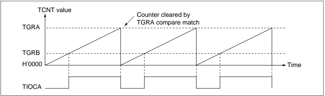
Figure 17.22 Example of PWM Mode Operation (1)
