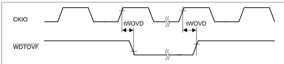
Figure 22.58 Watchdog Timer Output Timing ( t_{Ecy}:t_{Pcyc} = 1:1 )
