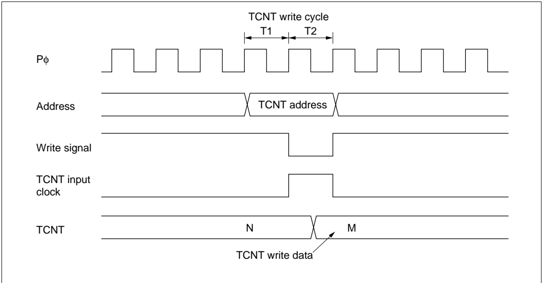
Figure 17.46 Contention between TCNT Write and Increment Operations
