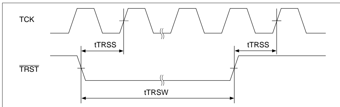
Figure 22.65 H-UDI \overline{\text{TRST}} Timing
