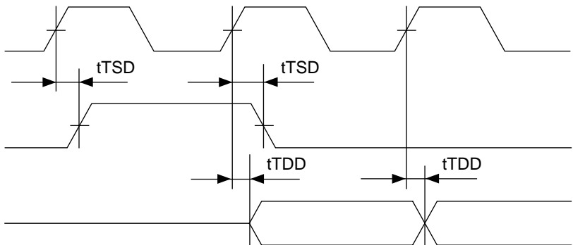
Figure 22.62 SIOF / SIO Transmit Timing (TMn = 0 Mode)
