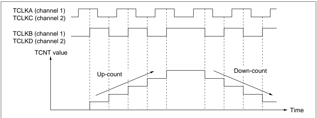
Figure 17.29 Example of Phase Counting Mode 4 Operation
