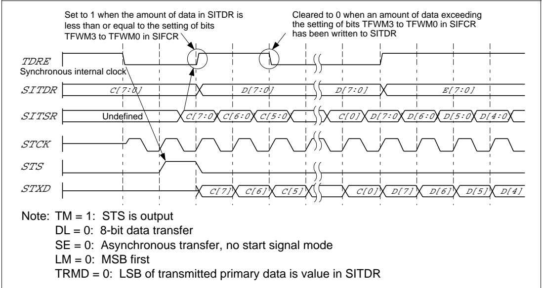
Figure 15.9 Transmission: Continuous Transfer Mode (TM = 1 Mode)/MSB First
