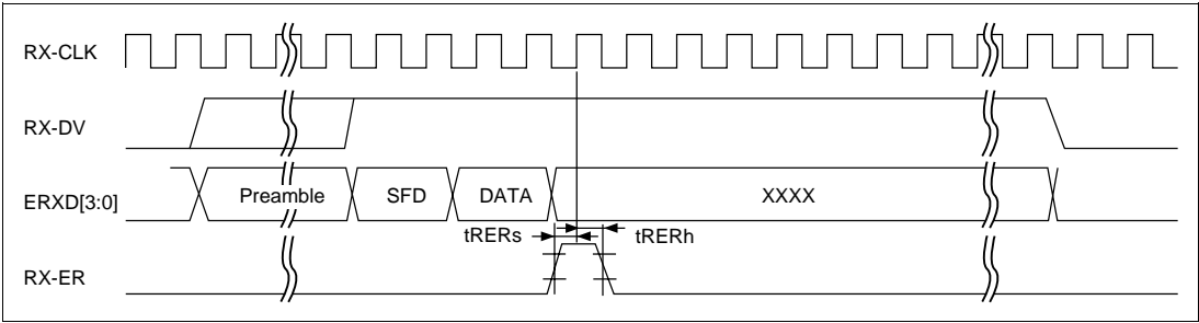
Figure 22.72 MII Receive Timing (Case of Error)
