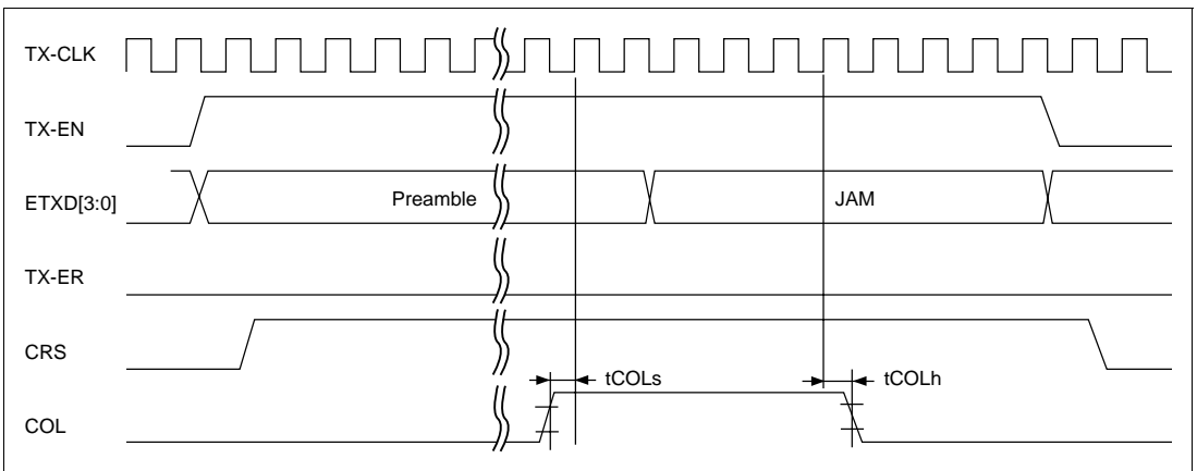
Figure 22.70 MII Send Timing (Case of Conflict)
