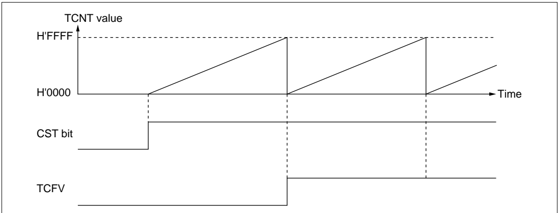
Figure 17.7 Free-Running Counter Operation
