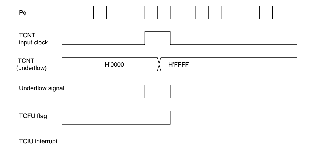
Figure 17.41 TCIU Interrupt Setting Timing
