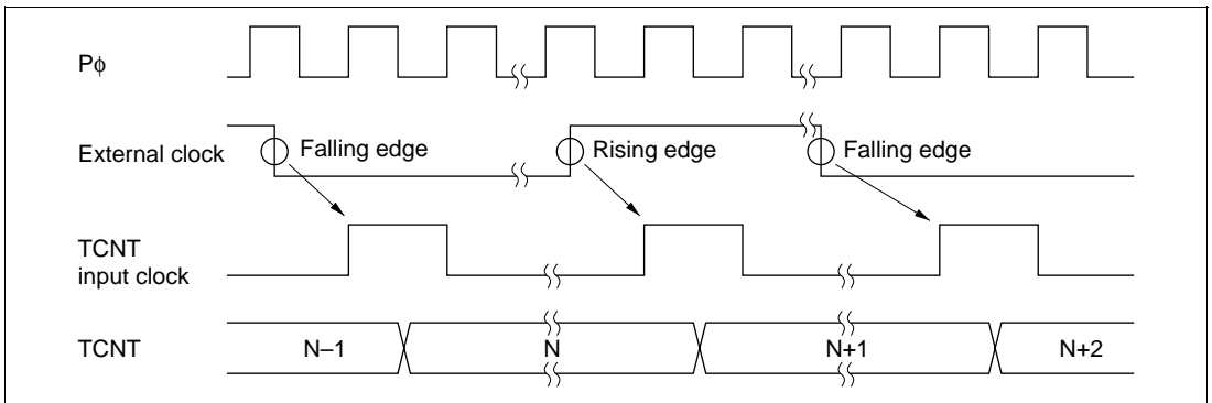
Figure 17.31 Count Timing in External Clock Operation
