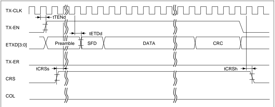
Figure 22.69 MII Send Timing (Normal Operation)
