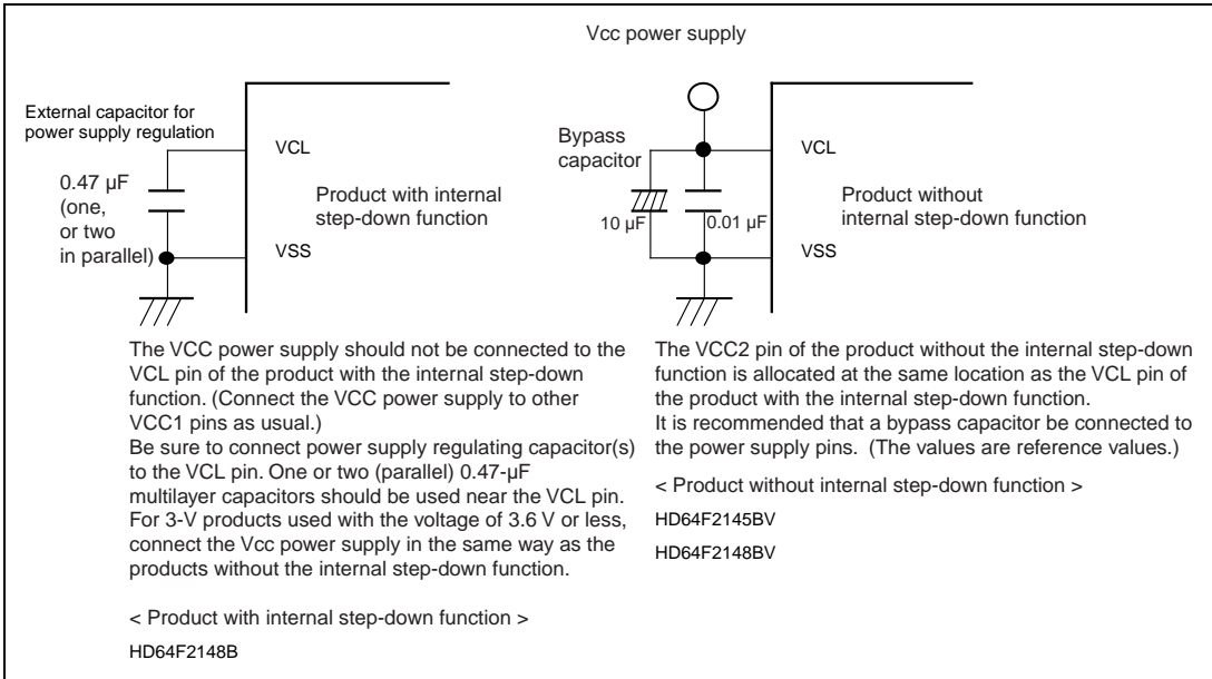
Figure 28.5 Connection of VCL Capacitor
