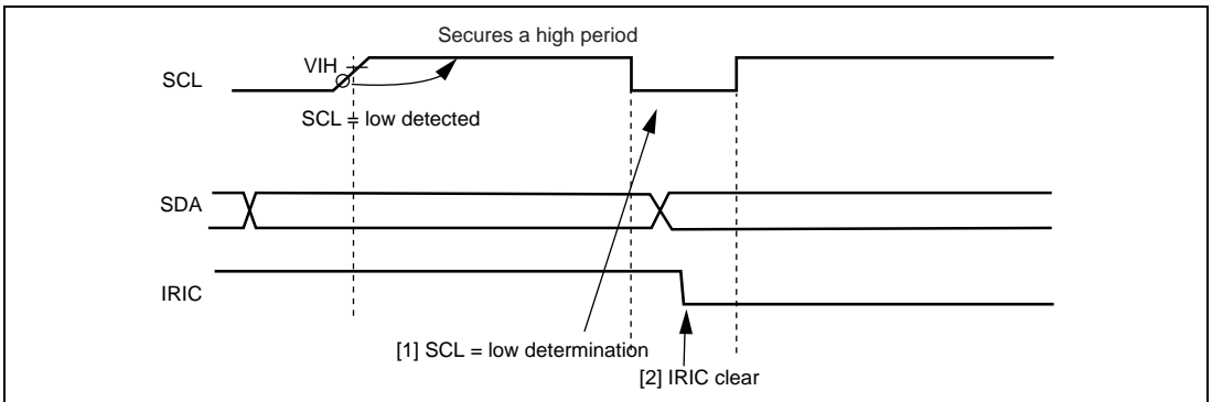
Figure 16.33 IRIC Flag Clearing Timing When WAIT = 1
