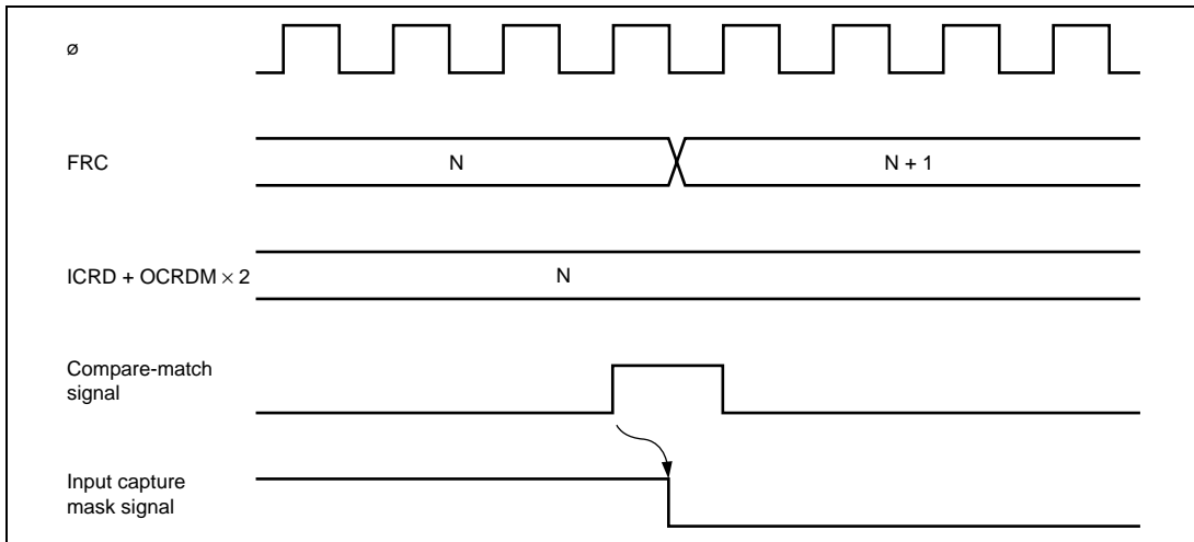
Figure 11.16 Timing of Input Capture Mask Signal Clearing
