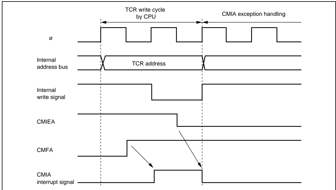
Figure 5.11 Conflict between Interrupt Generation and Disabling
