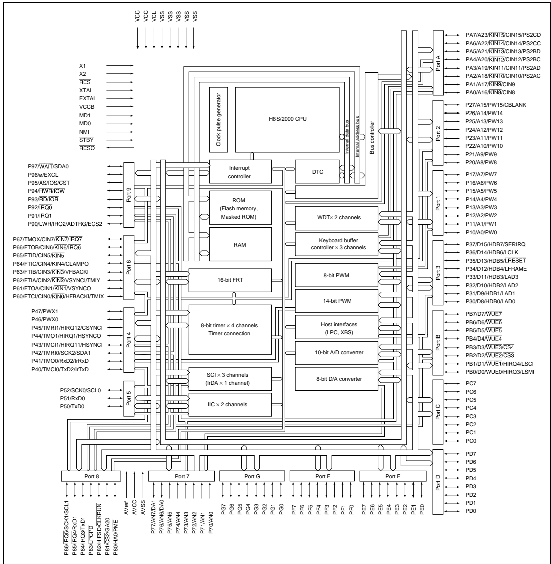
Figure 1.2 Internal Block Diagram of H8S/2160B and H8S/2161B
