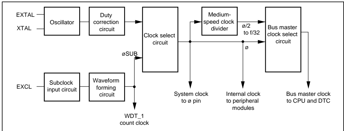
Figure 25.1 Block Diagram of Clock Pulse Generator
