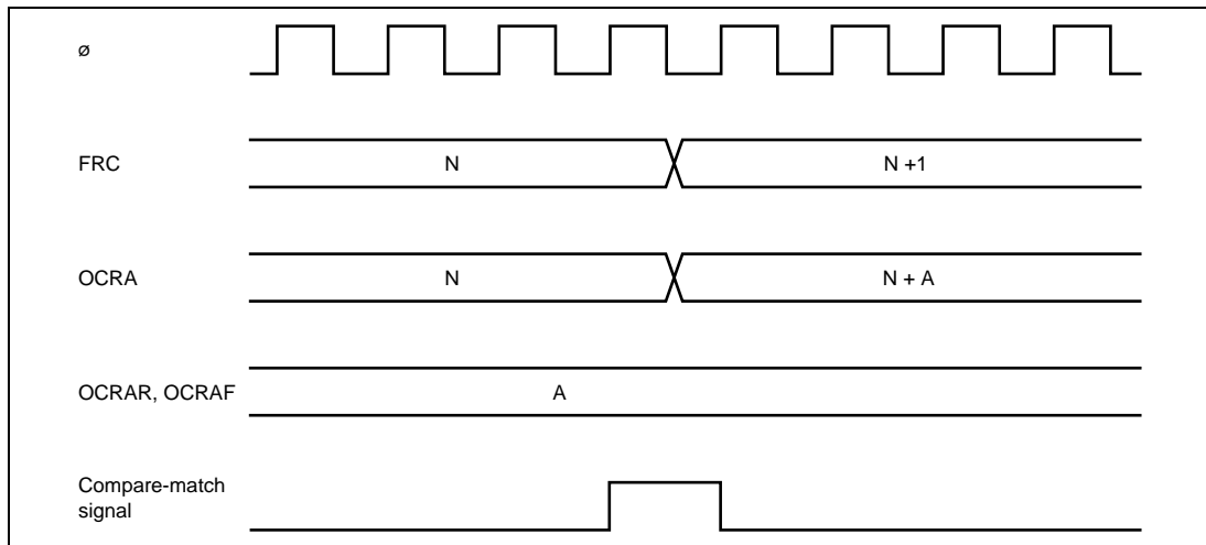
Figure 11.14 OCRA Automatic Addition Timing
