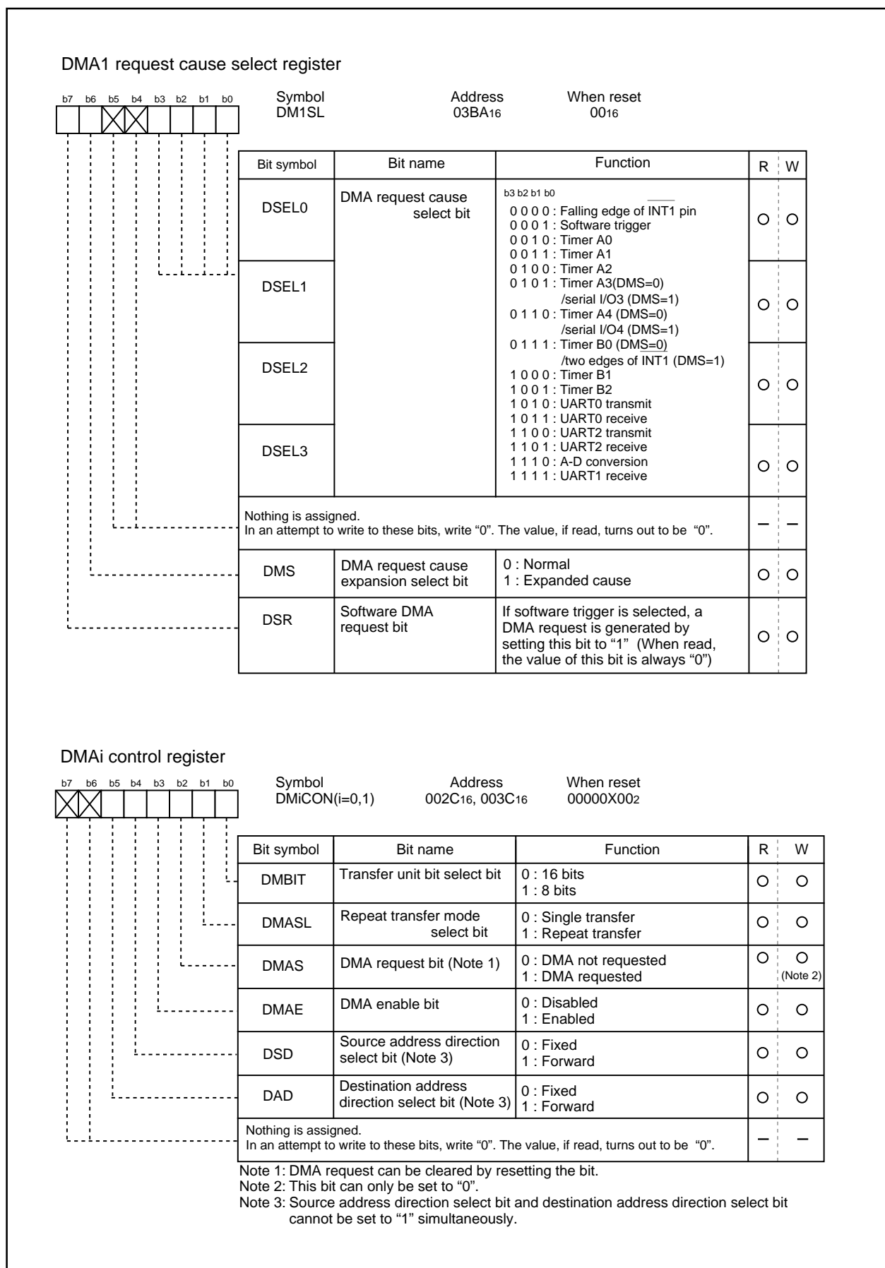
Figure 1.14.3. DMAC register (2)
