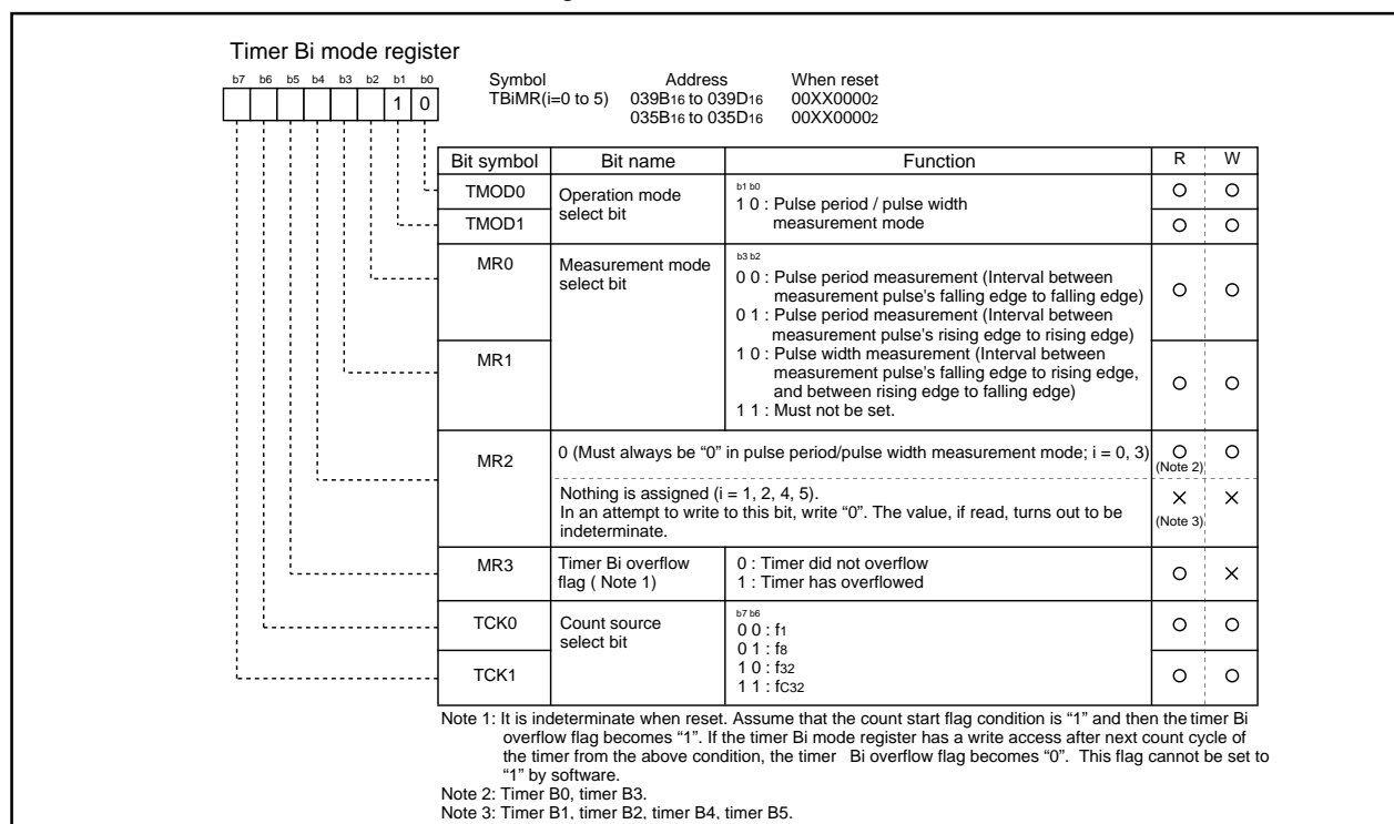
Figure 1.15.19. Timer Bi mode register in pulse period/pulse width measurement mode
