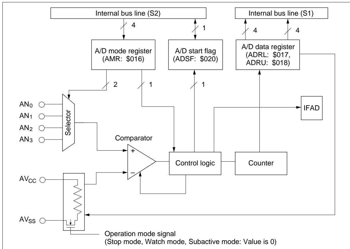
Figure 34 A/D Converter Block Diagram
