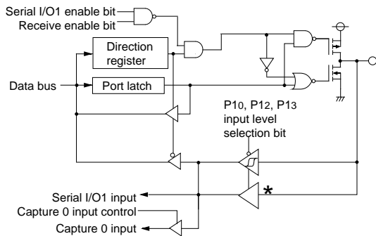
(8) Port P1 0
