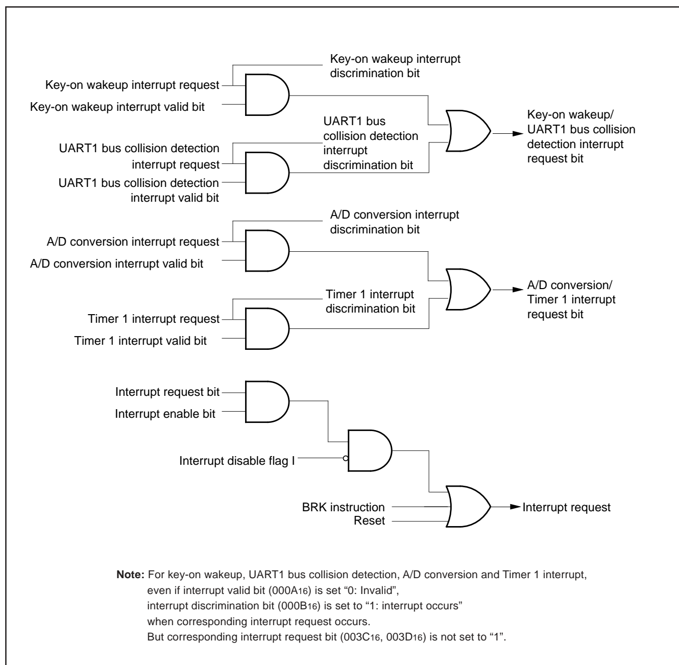
Fig. 23 Interrupt control
