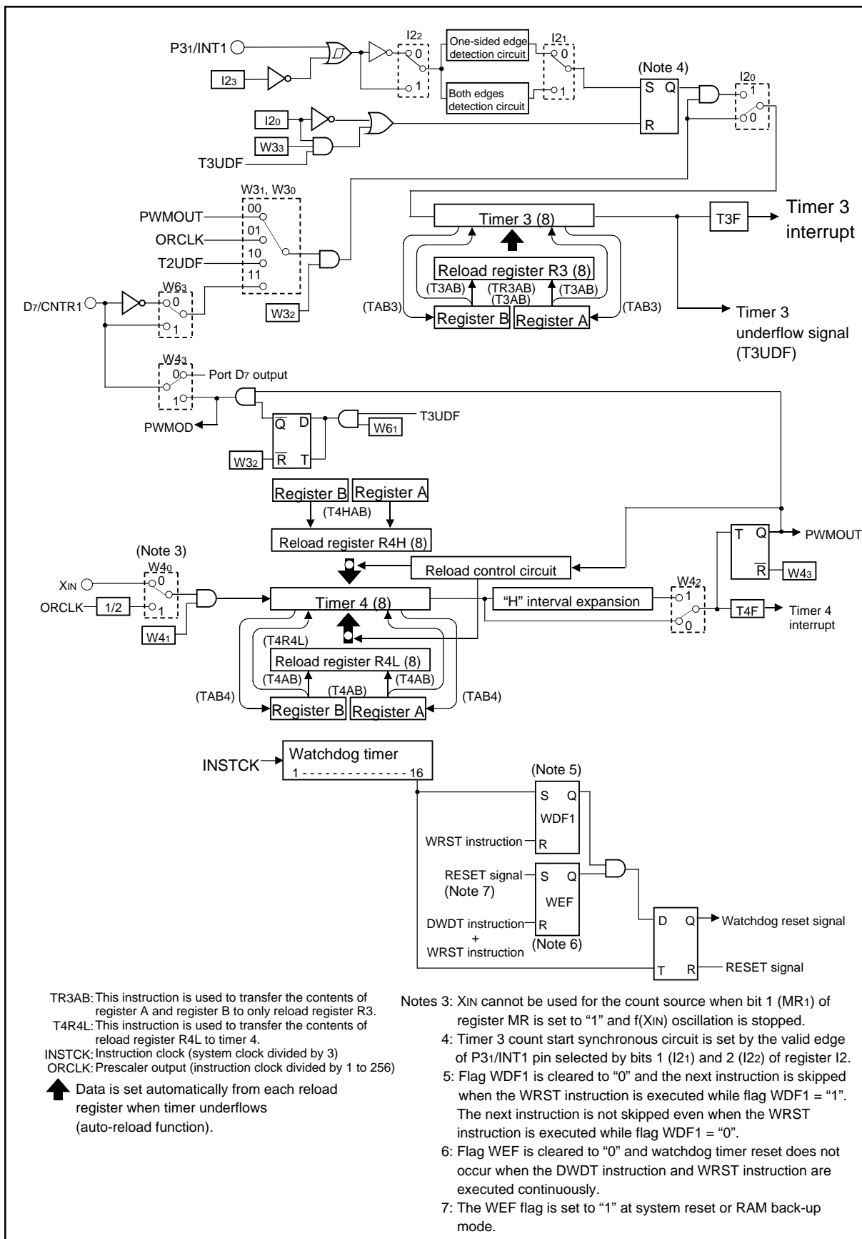
Fig. 26 Timer structure (2)
