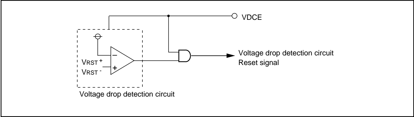
Fig. 49 Voltage drop detection reset circuit
