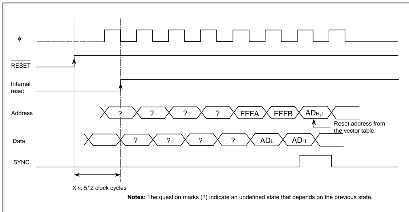
Fig. 54 Reset sequence
