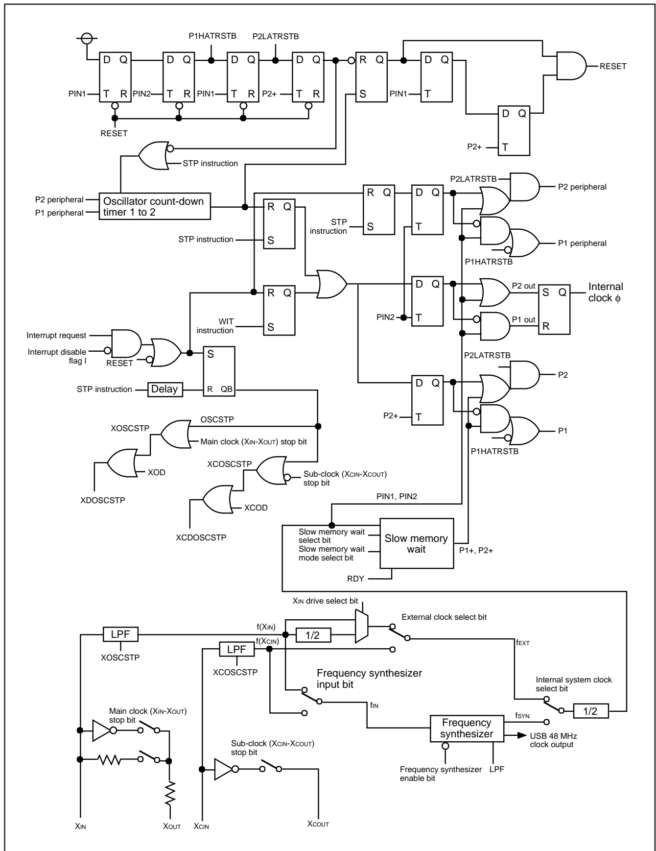
Fig. 59 Clock generating circuit block diagram
