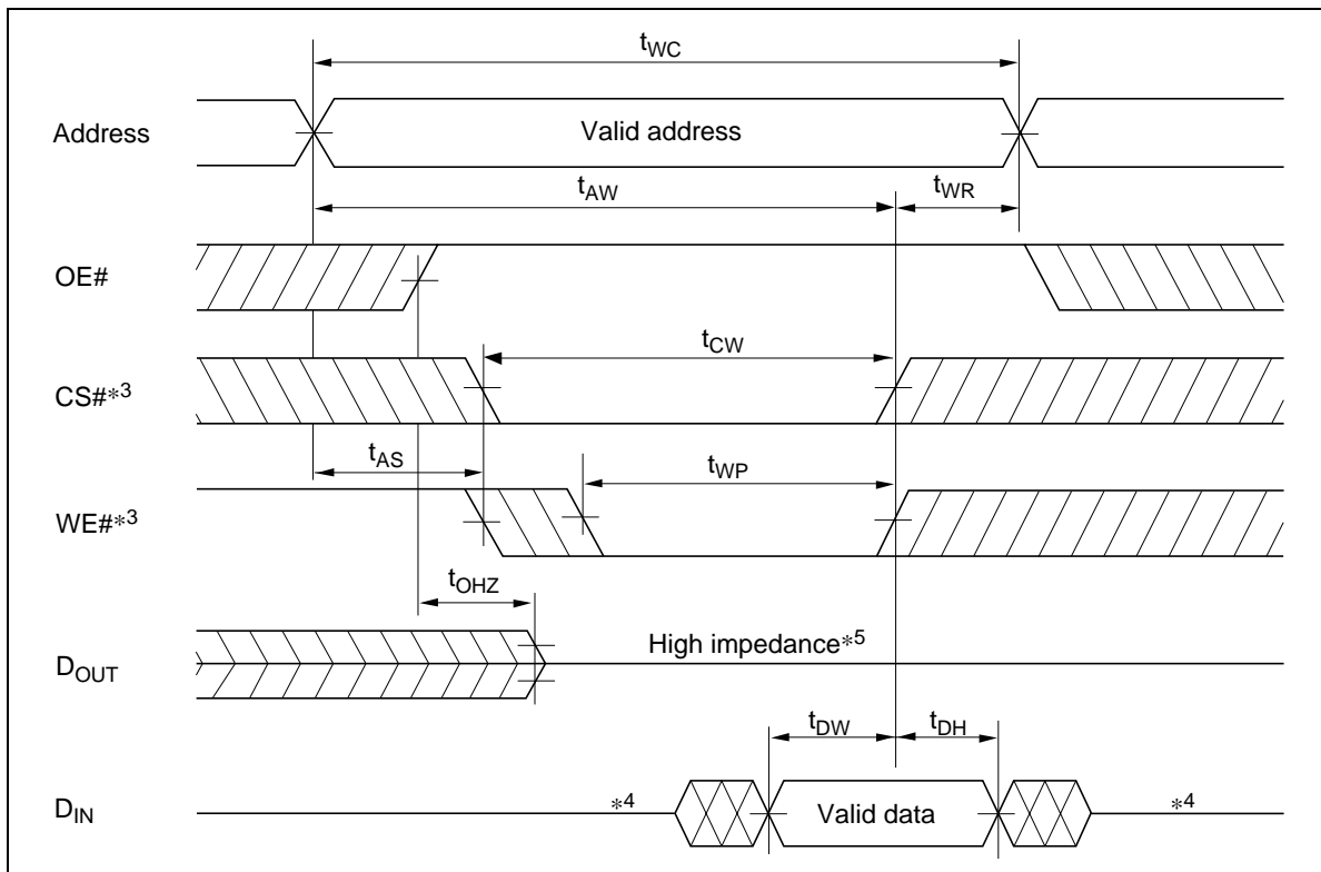
Write Timing Waveform (1) ( WE\# Controlled)
