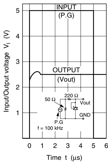
Pulse Response
